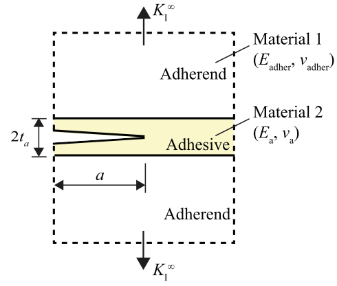
(b) F. Van Loock, M.D. Thouless, N.A. Fleck (2019) [14]: adhesive joint with semi-infinite crack subjected to a remote mode I K -field.
