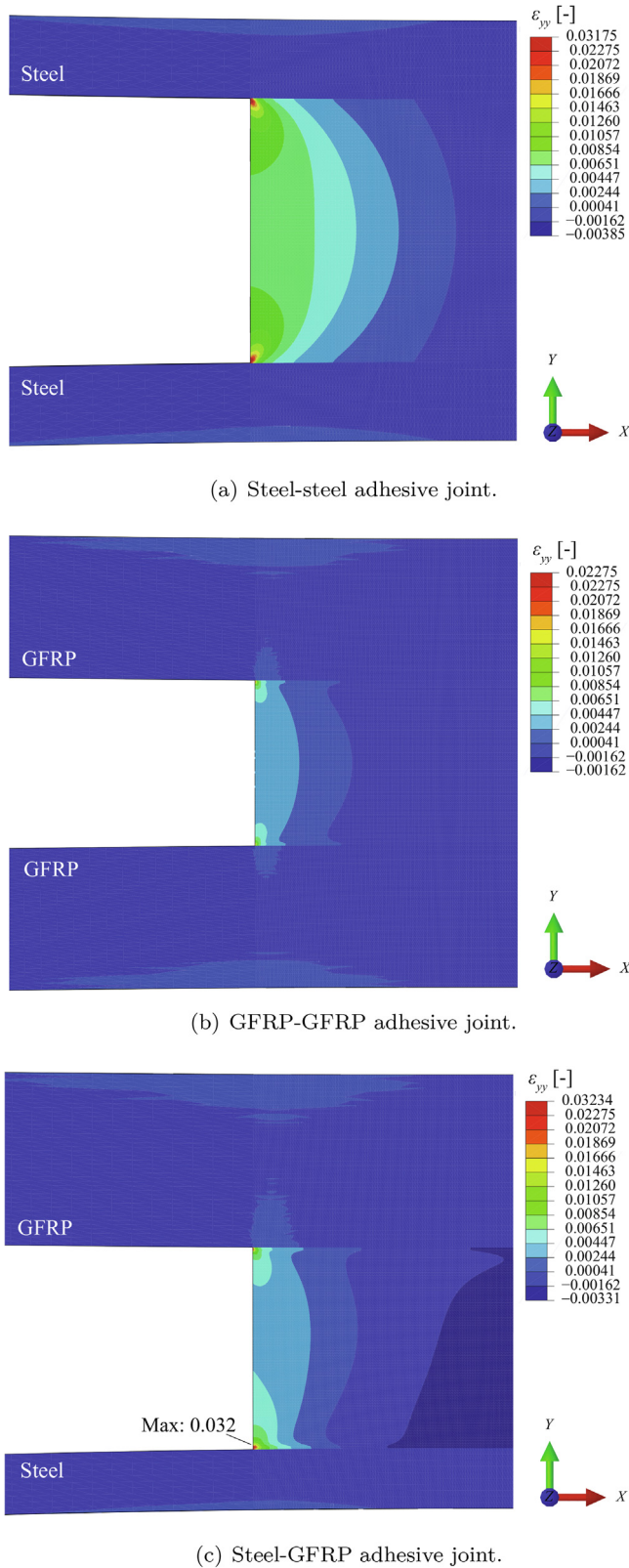
Fig. 13. Evolution of strain field, \varepsilon_{yy} , for different adhesive joint configurations and corresponding adherends-adhesive modulus-mismatches. No pre-crack is modelled, \Delta a = 0 mm, and same load is applied in all models. The results are taken along the mid-width of the model ( B = 0 mm).
