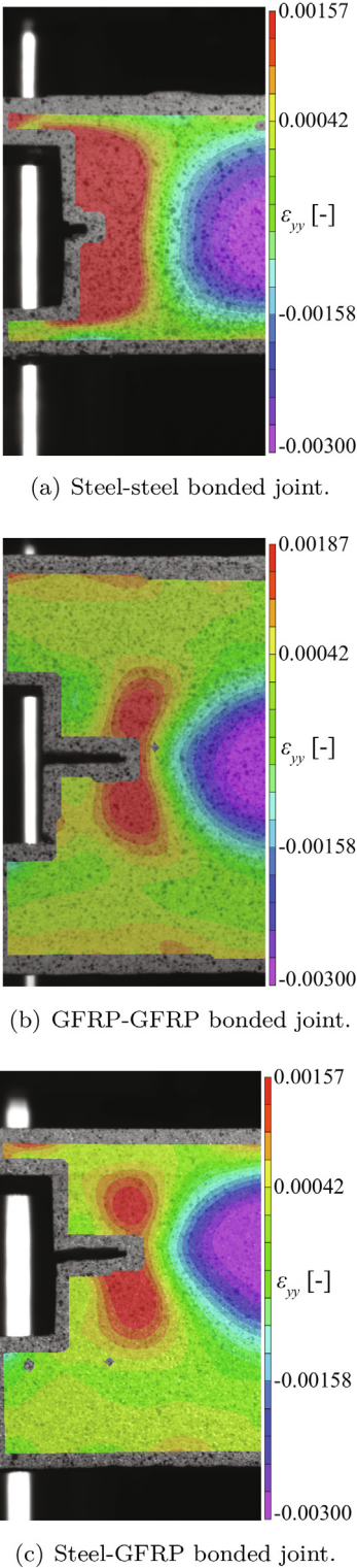
Fig. 15. Strain, \epsilon_{yy} , contour at fracture onset moment for three different specimens.
