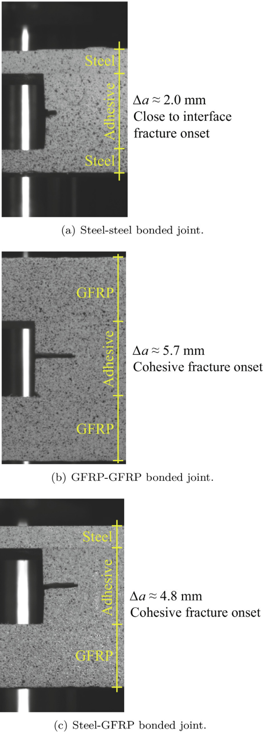
Fig. 14. Examples of experimentally investigated \Delta a 's.
