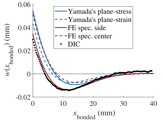
(b) Fracture onset moment.
