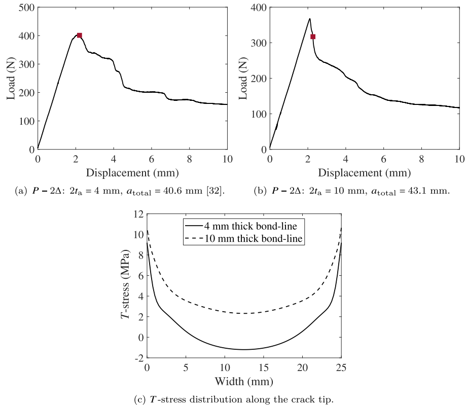
Fig. 19. Experimental load vs. displacement ( P-2\Delta ) curves and T -stress distribution at crack tip for DCB steel-steel specimens with different bond-line thicknesses.
