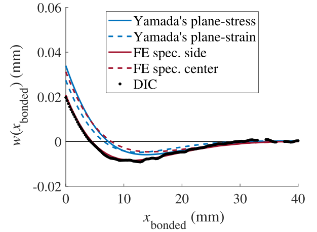
(a) Linear elastic region.
