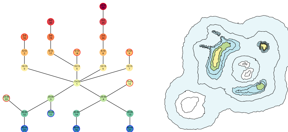
c) Region graph (nodes are areas, edges are isobaths) d) IHO coloured depth areas (nodes)
