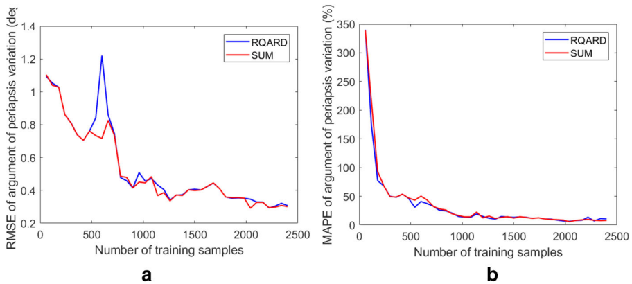
Fig. 13 The \omega error of test samples when the training dataset has a random sampling. The periapsis of initial osculating orbit of the spacecraft is outside the sphere of influence of the secondary. The best MAPE obtained is 5.7%
