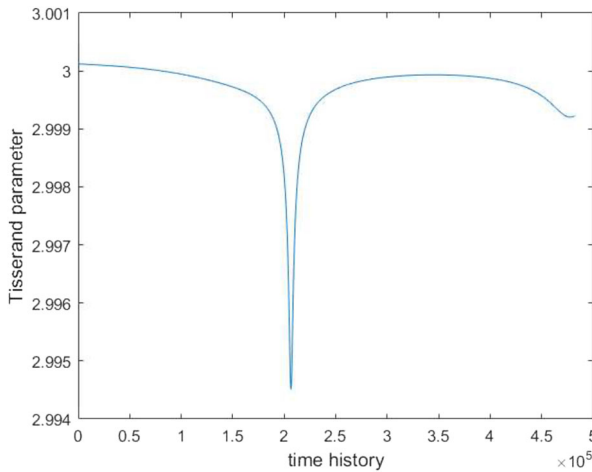
Fig. 4 The evolution history of the Tisserand parameter for the trajectory of Fig. 3. The X-axis shows the steps of the numerical integration for one orbital period
