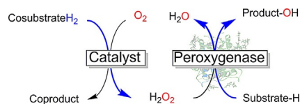
Scheme 10. Simplified scheme for peroxxygenase-catalysed oxyfunctionalisation reactions exploiting the oxygen dilemma.
