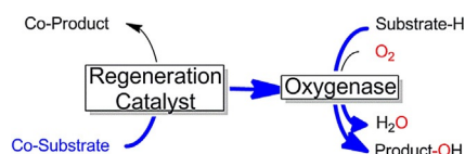
Scheme 7. Simplified regeneration of (mono)oxygenses by direct reductive regeneration of the enzymes' active sites.
