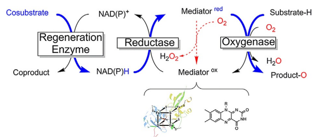
Scheme 4. Simplified molecular architecture of multicomponent monooxygenases that are not directly dependent on NAD(P)H. Blue: path of reducing equivalents. NAD(P)H serves as a general reductant, transferring its reducing equivalents to a mediator molecule (either a flavin or an iron-sulfur cluster protein) with catalysis by a reductase. The usually protein-based mediator delivers the reducing equivalents to the monooxygenase subunit for productive oxygen activation. However, direct reaction of the reduced mediator with \text{O}_2 leads to futile reoxidation and (eventually) \text{H}_2\text{O}_2 formation.
