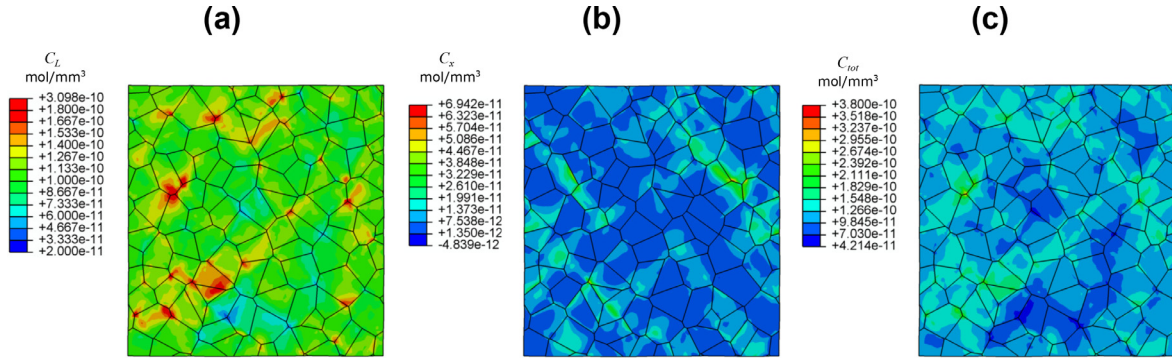
Fig. 8. The distribution of hydrogen in a RVE for HSS at 1000 bar of hydrogen pressure after 3 \times 10^{-2} tensile strain.
