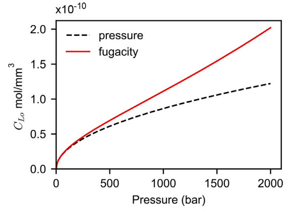
Fig. 3. The effect of pressure and fugacity on the equilibrium initial lattice concentration C_{Lo} of unstressed sample at 300 K.
