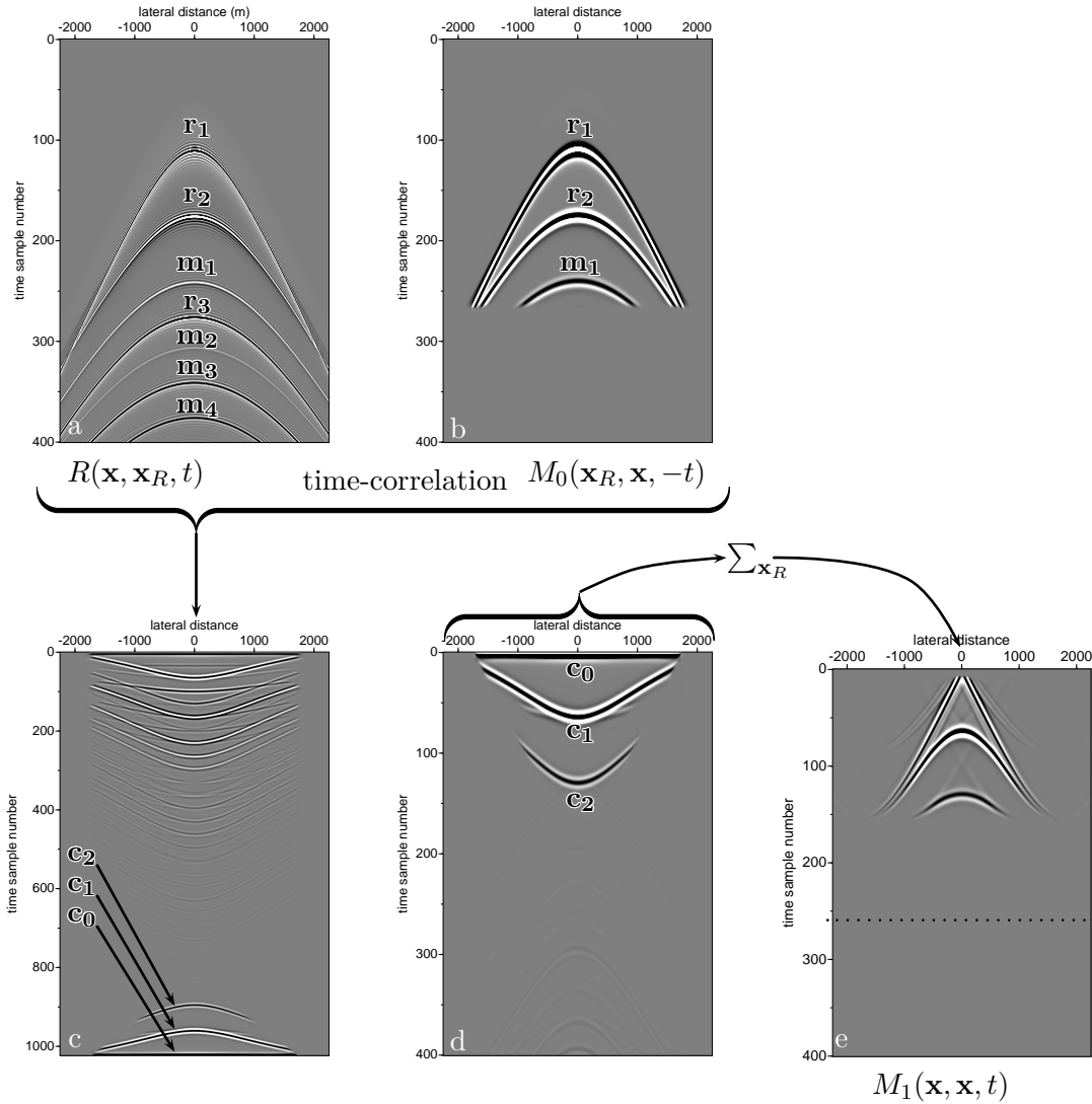
Figure 3: Computational steps to compute M_1 from M_0 at time sample number 276. The middle shot record from R is shown in (a); time truncated after sample 276 - n_\epsilon , and convolved with a Ricker wavelet, it gives M_0 in (b). Time-correlation of (a) with (b) gives (c). After time-reversal of (c) and applying the time window again gives (d). The traces in (d) are summed together and only the stationary point of events above sample 276 - n_\epsilon will end-up in the middle trace of M_1 (e). The mute window n_\epsilon samples later than t = 0 is needed to mute the autocorrelation of the first-event. The labeled events \mathbf{r}_i indicate the i 'th reflector and \mathbf{m}_l the l 'th multiple. In (c) the labeled correlated events are \mathbf{c}_0 = \mathbf{r}_1^* \cdot \mathbf{r}_1 + \mathbf{r}_2^* \cdot \mathbf{r}_2 + \mathbf{m}_1^* \cdot \mathbf{m}_1 , \mathbf{c}_1 = \mathbf{r}_2^* \cdot \mathbf{r}_1 + \mathbf{m}_1^* \cdot \mathbf{r}_2 , and \mathbf{c}_2 = \mathbf{m}_1^* \cdot \mathbf{r}_1 .
