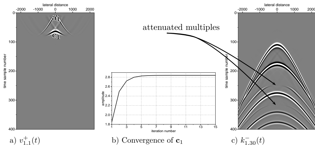
Figure 6: Creation of the event (labeled \mathbf{c}_1 ) that annihilates all the internal multiples between the first and second reflector, the artifact \mathbf{a}_1 is ignored in the analysis. Picture a) shows v_{1,1}^+(t) for the first Marchenko iteration at sample number ii = 200 . In b) the convergence of the maximum amplitude in \mathbf{c}_1 is shown as function of the iteration count. Figure c) shows the annihilated multiples in k_{1,30}^-(t) after 30 iterations.
