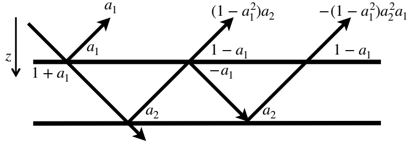
Figure 7: Sketch of the ray-paths and reflection and transmission coefficients in a three layer constant velocity and variable density model. The local reflection coefficients of the first and second reflector are a_1 and a_2 respectively.
