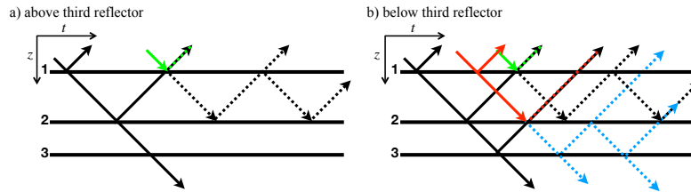
Figure 12: Compensation of internal multiples by events (coloured lines) that are created by the Marchenko method, applied for a point above (a) and below (b) the third reflector. The three reflectors are numbered from top to bottom.
