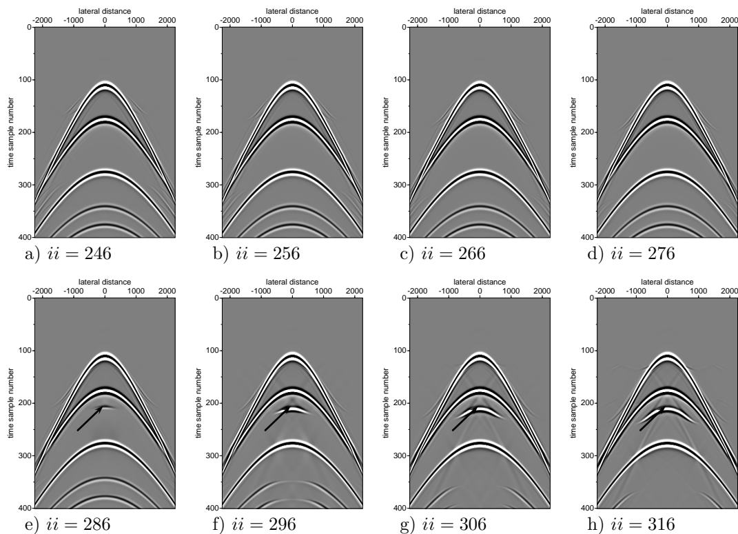
Figure 11: k_1^- after 32 iterations with different time instants ii = 246 to ii = 316 with steps of 10 samples. From each panel a constant-time cross section is selected at ii and all these cross-sections make up the multiple-free data. The arrows point to an event that compensates all internal multiples created between the second and third reflector.
