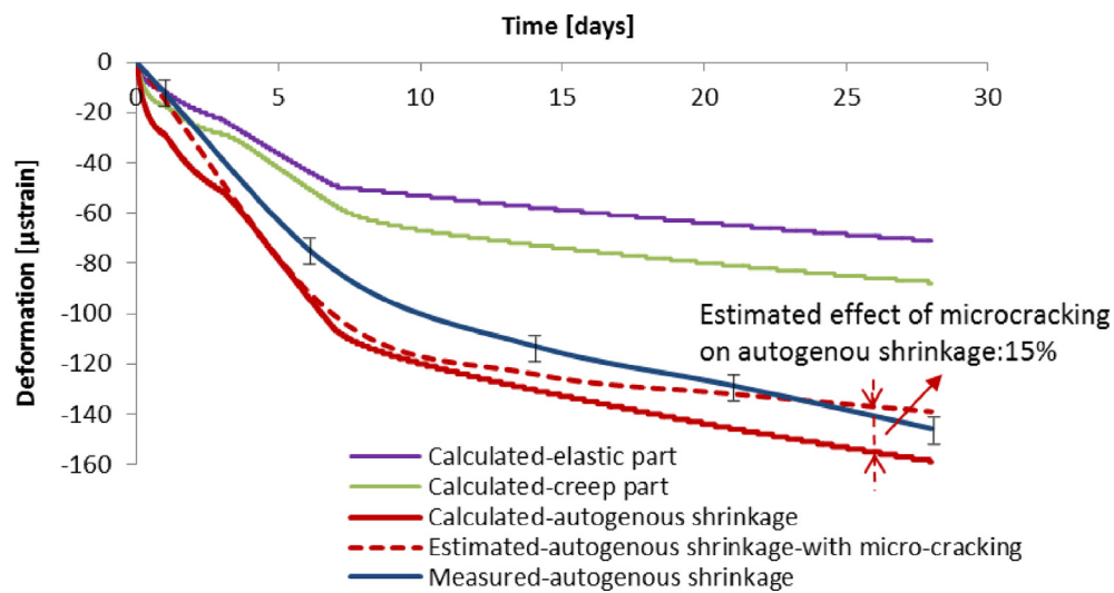
Fig. 28. Measured and adjusted calculated autogenous shrinkage of BFS concrete with w/b 0.44.
