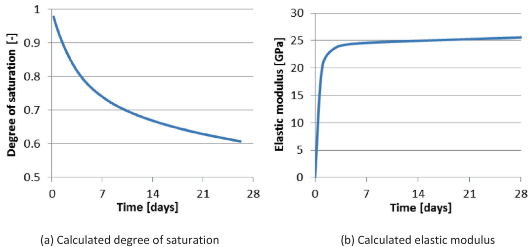
Fig. 21. Calculated degree of saturation and elastic modulus (with HYMOSTRUC) of Portland cement concrete.
