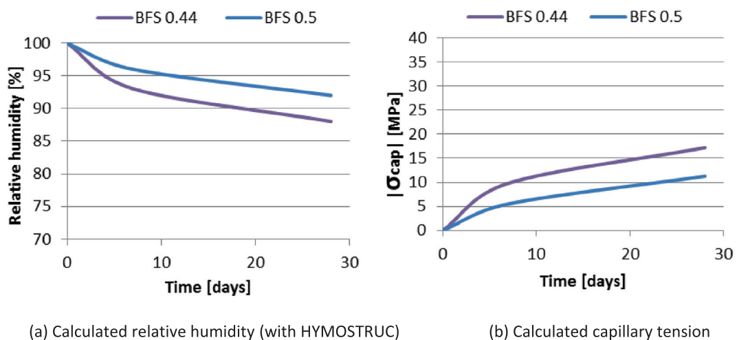
Fig. 23. Calculated relative humidity and capillary tension of BFS concretes.
