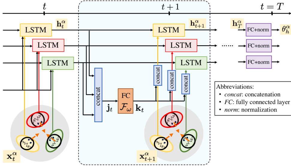
Fig. 2. Graphical illustration of our approach for head orientation estimation in the group context.
