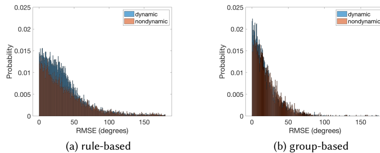
Fig. 8. RMSE distribution of Day 1 validation results using the rule-based and the proposed group-based approach.
