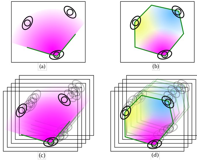
Fig. 3. Conceptual visualization of the motivation behind different methods. (a) The inputs and output are designed from an individual’s perspective in the group. The frame-based method is designed for this scenario. (b) The inputs and outputs are designed from a group perspective. (c) A sequential version of (a) where the change of interaction space in time is modeled using the sequence-based method (d). The proposed method, which is group-based, considers the change of the joint interaction space given that individuals influence each other during the course of an interaction.
