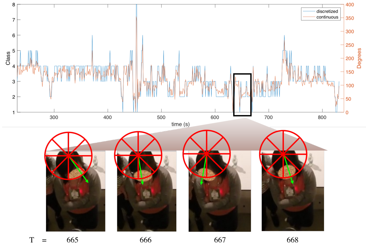
Fig. 6. Illustrative example of how small but noticeable head turns could result in the same class bin, resulting in a loss of fine-grained information. From T=665 to T=666 , the head turn with a relatively large magnitude resulted in the same bin. However, from T=666 to T=667 , a head with a smaller magnitude resulted in different bins.
