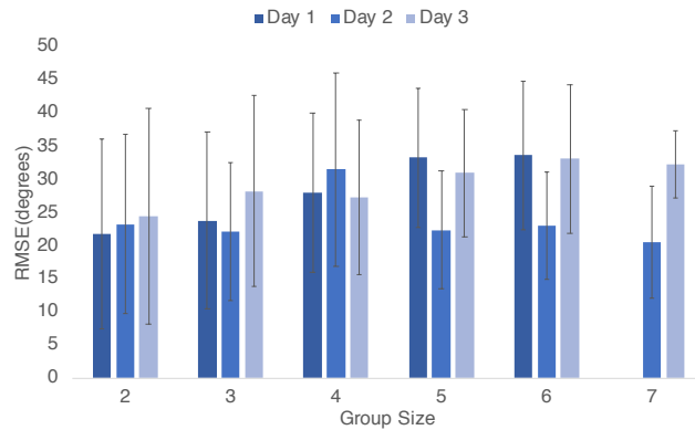
Fig. 7. Group-size-wise performance of the proposed group-based method in head orientation estimation. Note that there are no groups with seven members in the Day 1.
