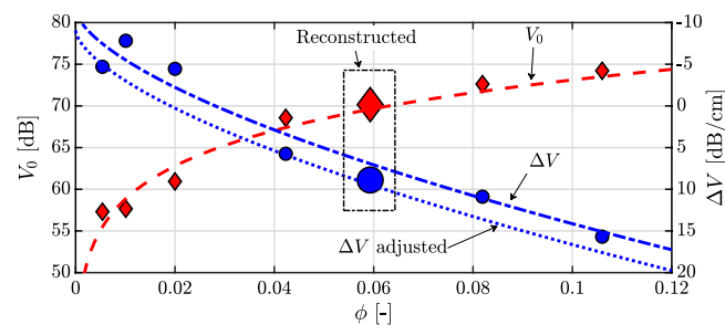
Fig. 10 Reconstruction of a step particle volume fraction profile. (Left) Calibration curves for the gelatin models, based on segment B. The larger symbols represent the characteristics of the case on which we apply stepwise reconstruction. (Right) Application of the stepwise reconstruction process to the phantom (segments B and C). For
