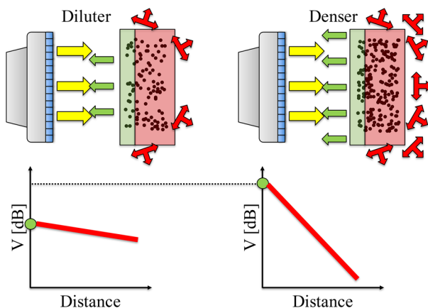
Fig. 3 Effect of particle loading on backscatter amplitude. For a fixedinsonification (yellow arrows pointing away from transducer), increasing the particle volume fraction in a uniform suspension increases the peak backscatter amplitude (green arrows pointing towards transducer in top panel and green circle in bottom, V_0 ) as the number of scattering interfaces are increased. However, the amount of scattering in the non-backscatter direction increases, leading to a quicker attenuation (groups of three red arrows originating from a node in top panel and solid red straight line in bottom, \Delta V ) of the backscatter amplitude
