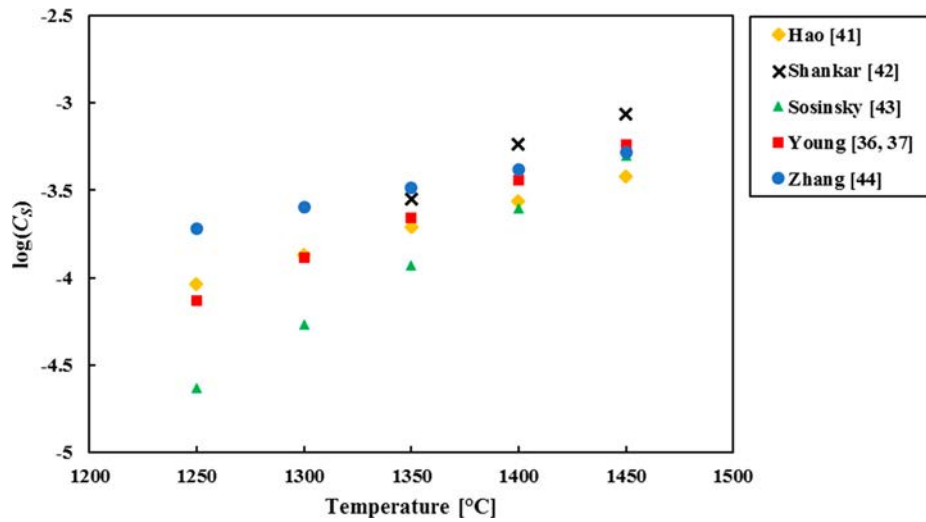
Figure 2. Comparison of C_S determined by the models from Table 3, for different temperatures.
