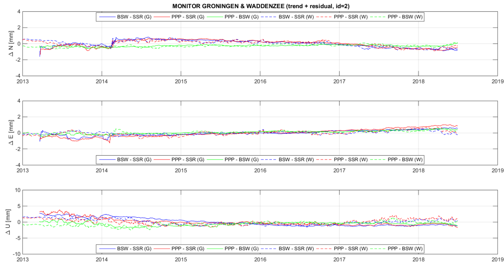
Figure 8.7: Trend differences for the Groningen (G) and Waddenzee (W) monitoring stations, after reference frame correction, for all combinations after 2013: SUM_TREND+RESIDUAL_NAM . The colored lines are time series of daily averages for the different combinations, the black lines are the moving 21 day median of the daily averages (with outlier and step detection).
