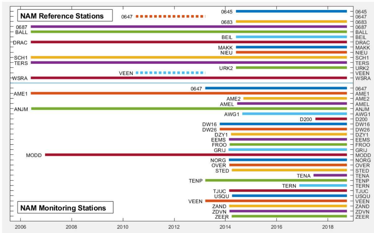
Figure 1.2: Timeline of NAM reference and monitoring stations. The stations VEEN and 0647 became monitoring stations in March 2013. Before March 2013 they were used as reference stations for GPS campaigns in the Waddenzee area, but, they have not been used as reference stations for the continuous stations AME1, ANJM or MODD.
