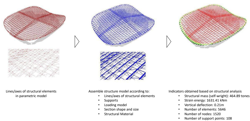
FIG. 3.7 An example about the assembly and analysis of a structure model based on Karamba 3d
