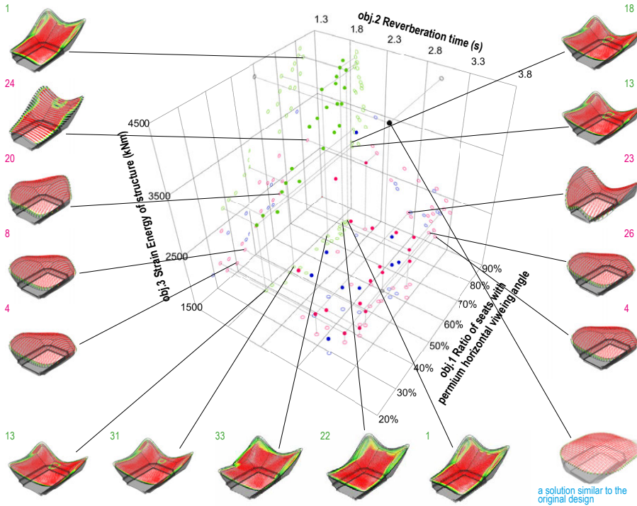
B. Comparison of the pareto solutions, a solutions similar to the original design, and some solutions selected from the iteration history of the optimization.
