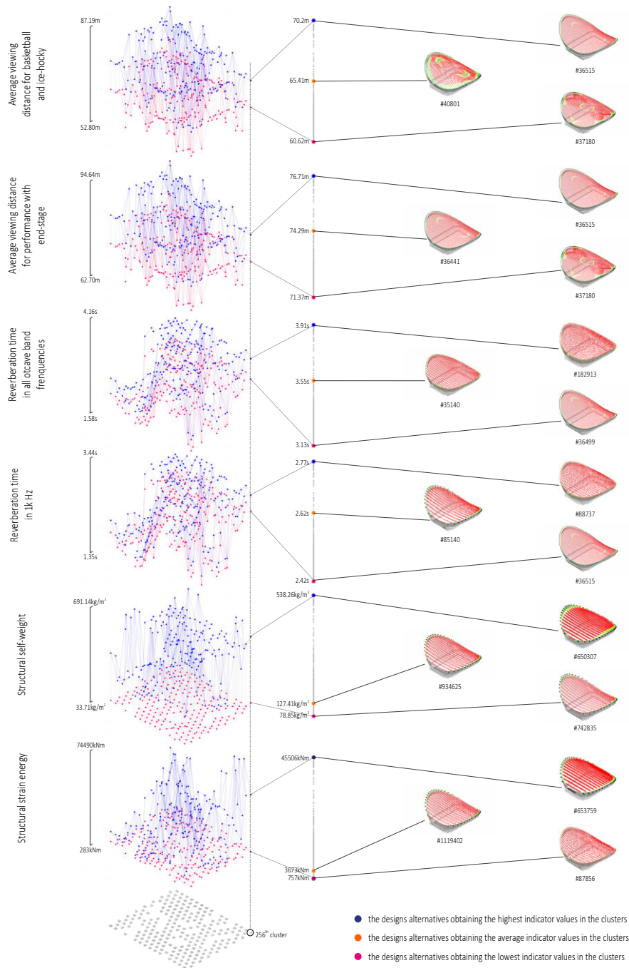
FIG. 5.18 Exploring the output spaces related to various quantitative indicators according to the design alternatives with different geometry types (design example of Barclay Centre)
