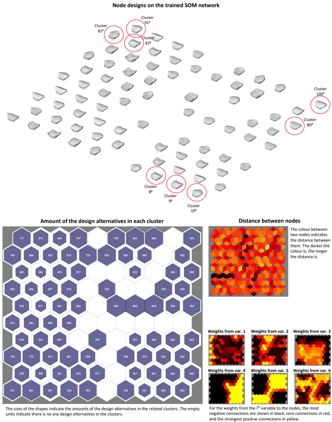
FIG. 5.7 The trained SOM network of the design space for the design example of Barclay Centre
