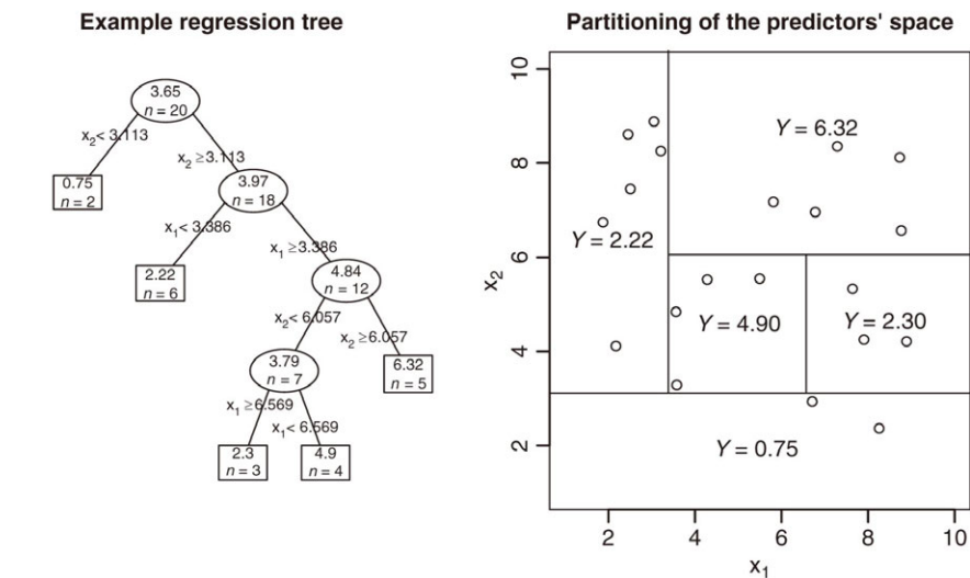
FIG. 3.12 A regression tree (left) and the related predictors' space (right) (Torgo, 2017)
