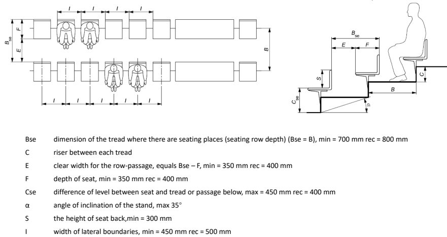
FIG. 2.8 The diagram of the regulations about seating tiers according to EN 13200-1:2012 (CEN, 2012)
