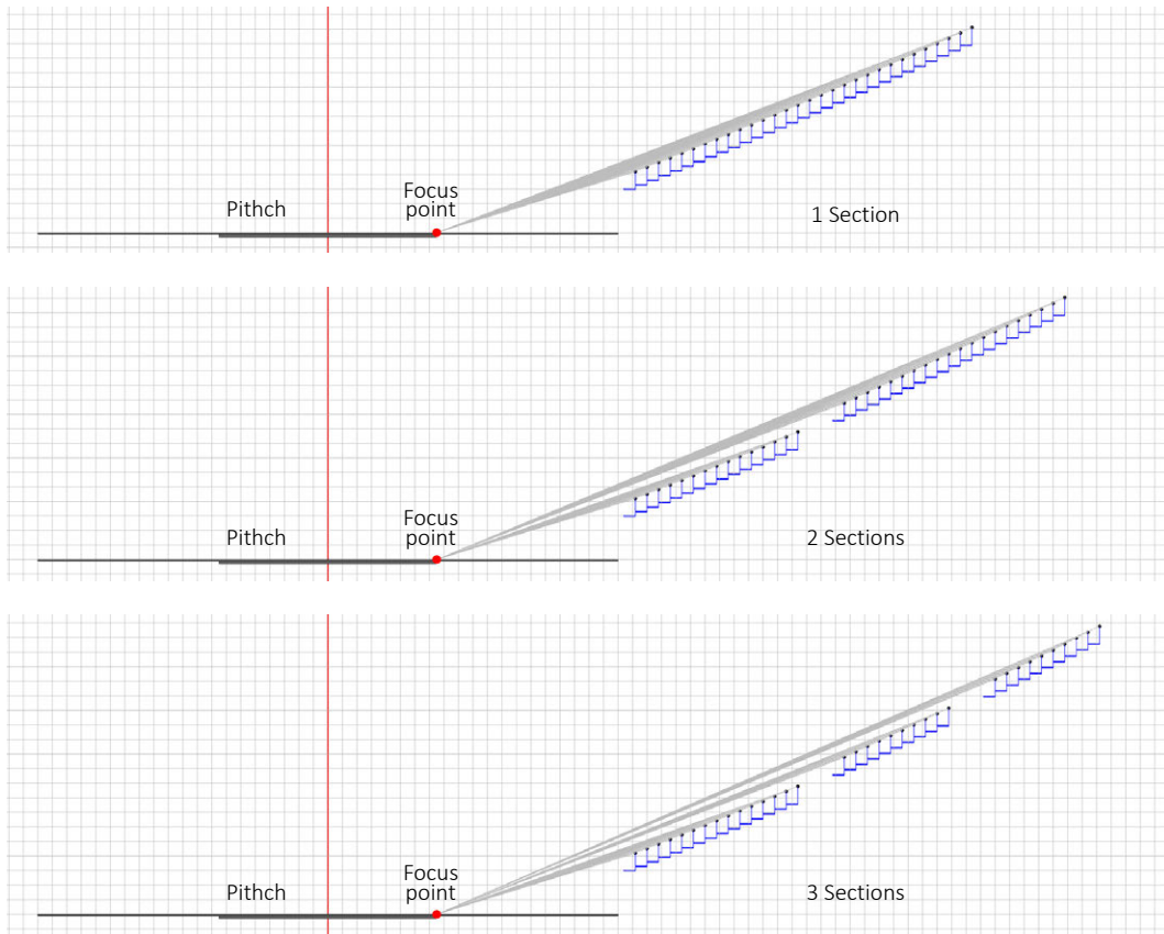
FIG. 2.13 Seating tiers divided into different sections
