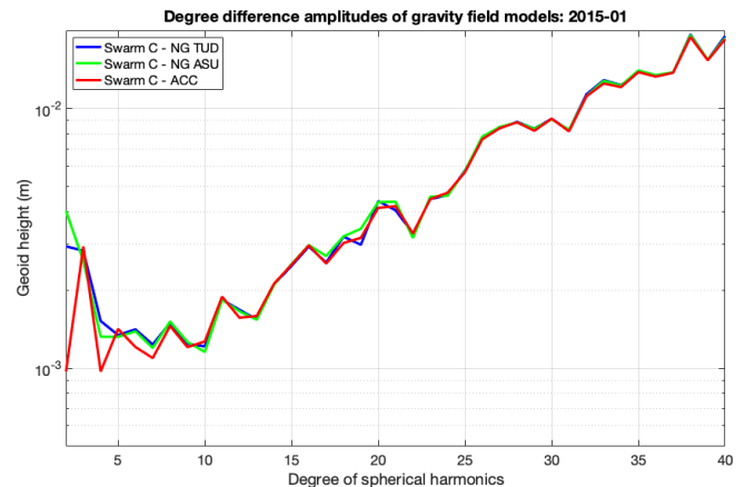
Figure 4. Swarm C gravity field solutions using TUD and ASU modelled non-gravitational accelerations, as well as measured non-gravitational accelerations (January 2015).
