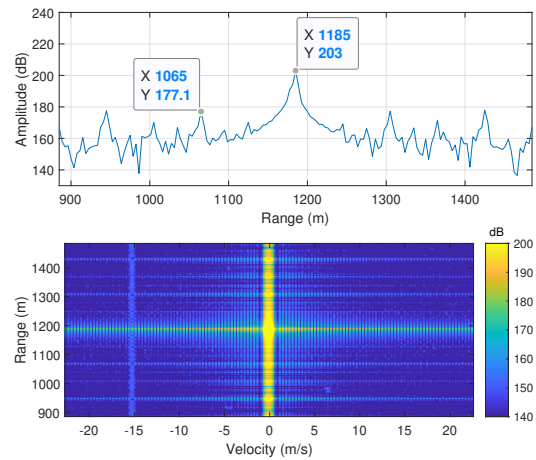
Fig. 8. Matched filter response for stationary target; range and range-Doppler map
