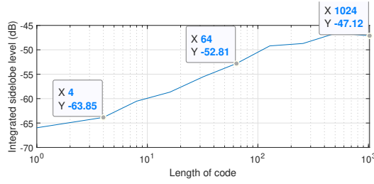
Fig. 3. Integrated sidelobe level vs the code lengths
