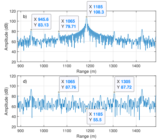
Fig. 6. Decoding simulation with the reference code away from the target; a) R = 5 m, b) R = 50 m, c) R = 100 m, d) R = 150 m
