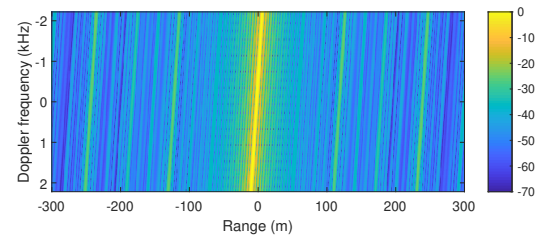
Fig. 1. Ambiguity function of the phase coded frequency modulated waveform for L_c = 1024 .
