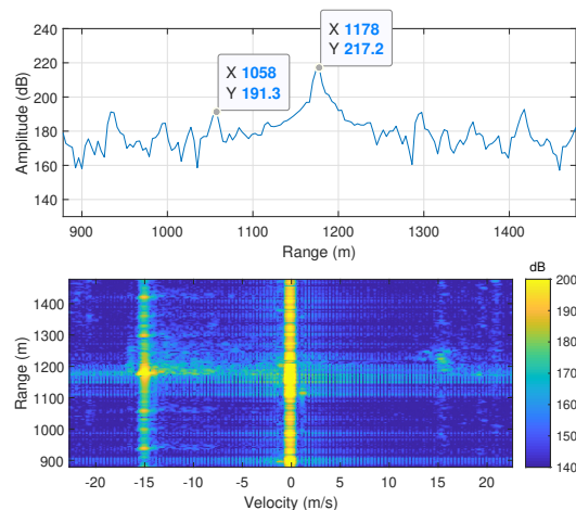
Fig. 10. Matched filter response for moving target; range and range-Doppler map
