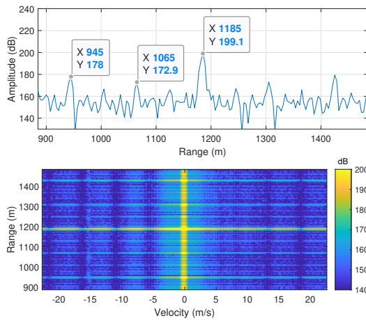
Fig. 7. Dechirping and decoding with reference delay R = 50 m for stationary target; range and range-Doppler map
