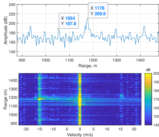
Fig. 9. Dechirping and decoding with reference delay R = 50 m for moving target; range and range-Doppler map
