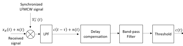
Fig. 4. Block diagram of communication
