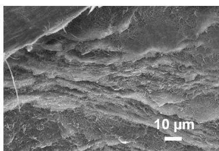
Figure S3.4 SEM image of 10 % PVA-BC sample, where no freezing-thawing procedure was carried out. It shows a similar structure to that of natural BC, with no special circular or honeycomb structure observed.
