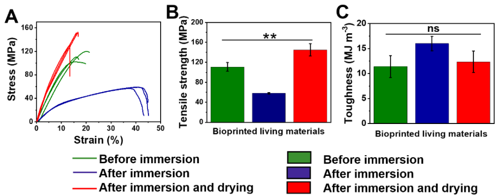
Figure S6.14 Tensile testing of bioprinted materials before and after immersion into water (A) stress-strain curves, (B) tensile strength, (C) toughness. ns, not significant; **p < 0.01 as determined by one-way (single factor) ANOVA with post-hoc Tukey's HSD.
