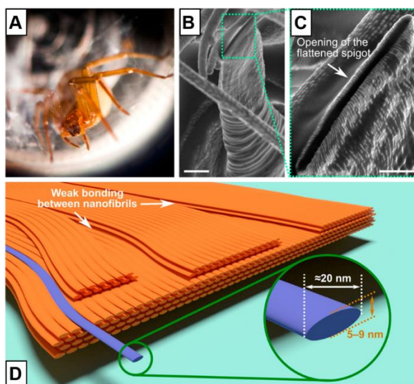
Figure 1.1 Nanofibrous layered structure of spider silk. (A-C) Spider ( Loxosceles laeta ) and the flattened Loxosceles spigot from which silk ribbons are extruded. (D) Scheme of the fibrous layered organization of a Loxosceles silk. Scale bars of (B) and (C) are 5 \mu\text{m} and 2 \mu\text{m} , separately. This image is reproduced with permission from ref 1 (Copyright 2018 American Chemical Society).
