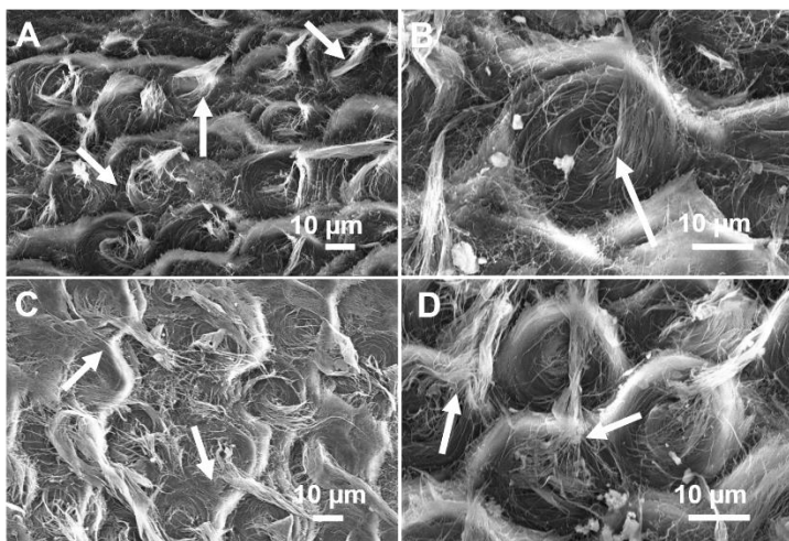
Figure S3.8 SEM images of the de-spiral morphology of the honeycomb specimen after failure (10 % PVA-BC-FT sample). The different panels (A-D) represent different magnifications. De-spiral morphologies (white arrows) are shown in all the images.
