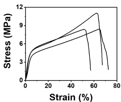
Figure S2.6 Tensile stress-strain curves of biomaterialized BC composites produced with 10 mM \text{Ca}^{2+} in the biomaterialization medium and without PGA.
