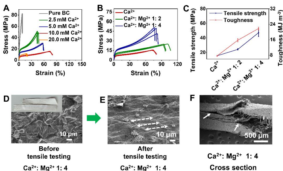
Figure 2.4 Mechanical properties of the biomineralized BC composites. (A) Tensile stress-strain curves of biomineralized BC with different \text{Ca}^{2+} content in the biomineralization medium. (B) Tensile stress-strain curves, (C) tensile strength, and toughness values of biomineralized BC with and without \text{Mg}^{2+} ions in the biomineralization medium. (D, E) Optical and SEM images of the surface morphology of the biomineralized BC composite with \text{Ca}^{2+}:\text{Mg}^{2+} ratio of 1: 4 (D) before and (E) after tensile testing. Arrows represent stretched sample wrinkles after the application of load. (F) SEM images of the cross-section of the biomineralized BC composite with \text{Ca}^{2+}:\text{Mg}^{2+} ratio of 1: 4 after tensile testing. Arrows indicate delamination in the specimen. All the samples in this figure were made with PGA.
