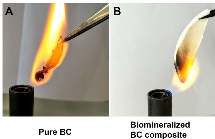
Figure S2.10 Optical images of (A) pure BC exposed to a flame for 1 second and (B) biomineralized BC composite ( \text{Ca}^{2+} : \text{Mg}^{2+} 1: 4) exposed to a flame for 1 minute. Due to the high inorganic crystal content, the biomineralized BC composite showed fire retardant abilities throughout 1 minute of direct exposure to the flame (B), while pure BC ignited immediately upon contact with the flame (A).
