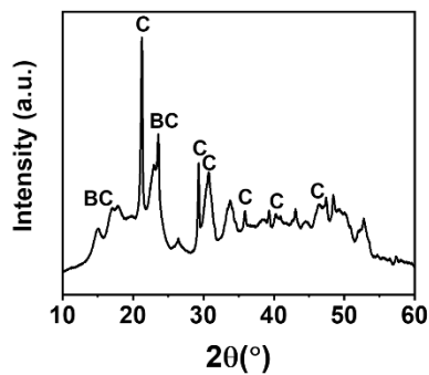
Figure S2.4 XRD spectra of the biomaterialized BC composite (Ca: Mg 1:4 with PGA). The \text{CaCO}_3 crystals in the final composite show a calcite (C) morphology.
