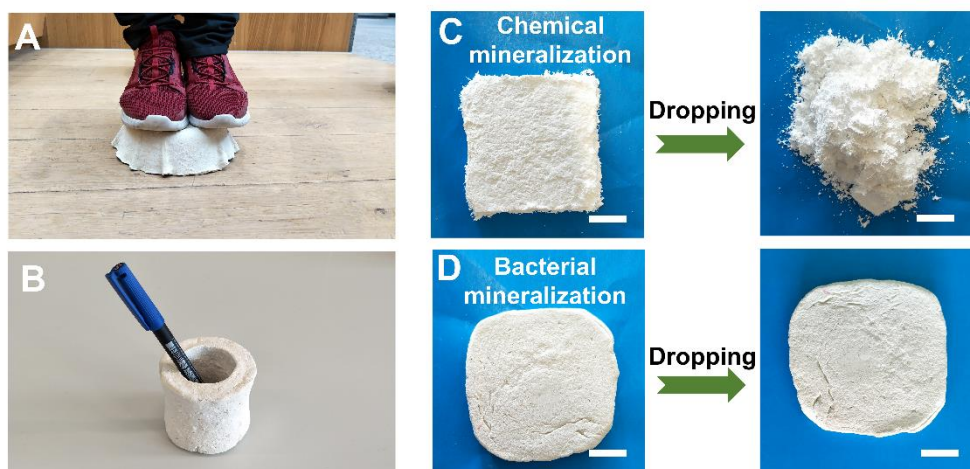
Figure 2.6 Examples for the applications of the biomineralized BC composites. Biomineralized BC composites ( \text{Ca}^{2+} : \text{Mg}^{2+} = 1: 4) molded into (A) a stool shape, and (B) a cup. Composites produced with the (C) chemical method and (D) bacterial biomineralization method before (left) and after (right) dropping from a 10 m height three consecutive times. All the samples in this figure were made with PGA. Scale bars correspond to 2 cm.
