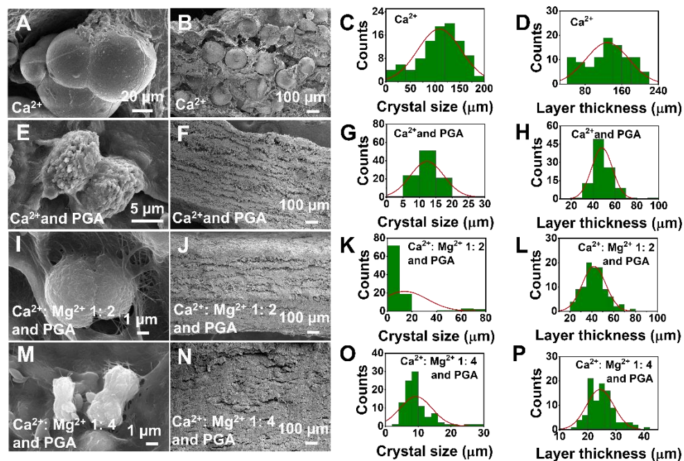
Figure 2.2 Morphology of biomaterialized BC composites. (A, E, I, M) Representative SEM images of crystals within the biomaterialized BC with (C, G, K, O) associated crystal size distributions. (B, F, J, N) SEM images of the material cross-sections and (D, H, L, P) layer thickness distributions of biomaterialized BC composites. Biomaterialized BC samples were fabricated either (A-D) without or (E-P) with PGA in the biomaterialization medium; and with either (A-H) only \text{Ca}^{2+} , or with a \text{Ca}^{2+} : \text{Mg}^{2+} ratio of (I-L) 1: 2 or (M-P) 1: 4 in the biomaterialization medium.
