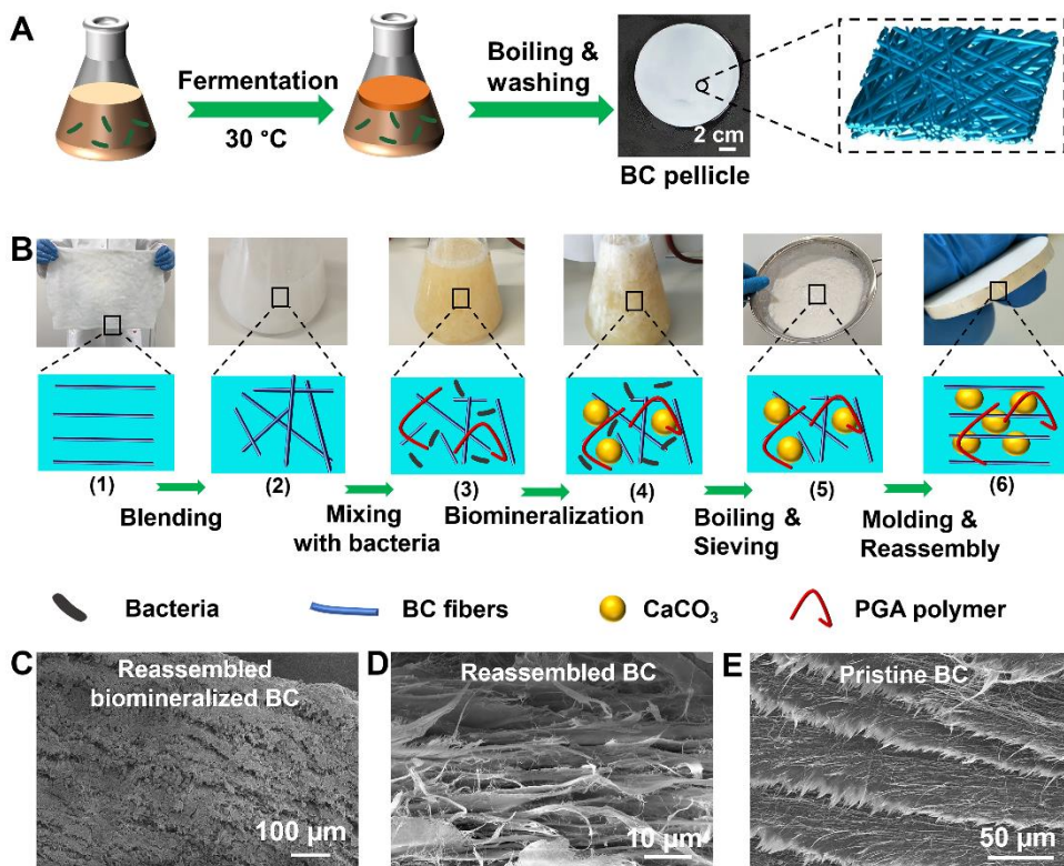
Figure 2.1 Biomaterialized BC fabrication. (A) Fabrication procedure of BC, including a static in situ fermentation at 30 °C, boiling with sodium hydroxide, and washing with distilled water. The BC pellicle shows a hydrogel-like appearance and a nano-fibrous layered microstructure. (B) Fabrication procedure of the biomaterialized BC, from step (1) to (6): (1) to (2) blending the BC hydrogel into a fibrous suspension, (2) to (3) mixing the BC fibrous suspension with the bacteria mineralization ingredients (CaCl 2 , urea, bacteria, medium, and PGA), (3) to (4) biomaterialization, (4) to (5) boiling and sieving the biomaterialized slurry to remove the bacteria and medium, (5) to (6) molding the purified biomaterialized BC slurry, and solvent-evaporation-induced self-assembly. The final material shown on the picture was polished with sandpaper. (C-E) Scanning electron microscope (SEM) images of the cross sections of (C) reassembled biomaterialized BC composite, (D) reassembled BC, and (E) pristine BC.
