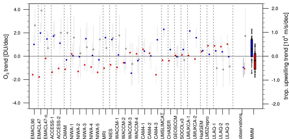
Figure 2. LS ozone trends and their uncertainties in the tropics ( 20^{\circ}\text{N} – 20^{\circ}\text{S} ; red dots) and northern mid-latitudes ( 30^{\circ}\text{N} – 50^{\circ}\text{N} ; blue dots) together with tropical upwelling trend (black circles; for all simulations providing TEM diagnostics) for the period 1998–2018 for all REF-C2 simulations. Dashed lines separate the individual models. Moreover, observational trends (1998–2018) and multi-model mean trends are given. Observational data for ozone are taken from BASIC SG and for tropical upwelling from ERA5 reanalysis. Error bars associated with each LS ozone trend represent the 90 % confidence intervals. The multi-model mean trends are shown as boxplots: the solid black line in the box indicates the median, the black point indicates the MMM, and the coloured box ranges from the 25th to the 75th percentile of the trends. Crosses denote trends of individual model simulations not lying within the box.
