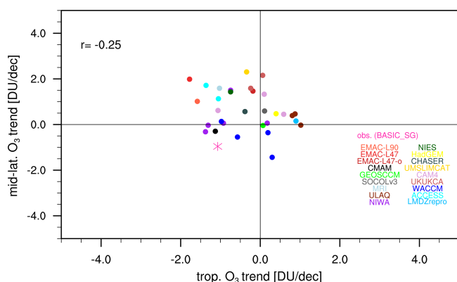
Figure 3. Inter-model correlation between tropical (20° S–20° N) and northern mid-latitude (30°–50° N) LS ozone column trends, calculated over the period 1998–2018 for 31 CCM REF-C2 simulations. All ensemble members of a particular model are shown in the same colour. The observational ozone trends (BASIC SG ) are included as a star.
