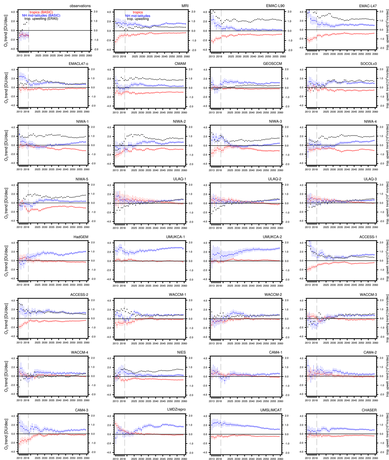
Figure 5. Tropical ( 20^{\circ} S– 20^{\circ} N) and northern mid-latitude ( 30^{\circ} – 50^{\circ} N) LS ozone column trend and their uncertainties (in DU per decade) of observations (BASICSG) and REF-C2 simulations as a function of the end year (red and blue dots, respectively). Tropical upwelling trends are included for all REF-C2 simulations where TEM diagnostics were available (black dots); observational tropical upwelling is taken from ERA5 reanalysis. The end year varies from 2013 to 2019 for observational data and from 2013 to 2060 for REF-C2 simulations. Error bars associated with each trend represent the 90 % confidence intervals.
