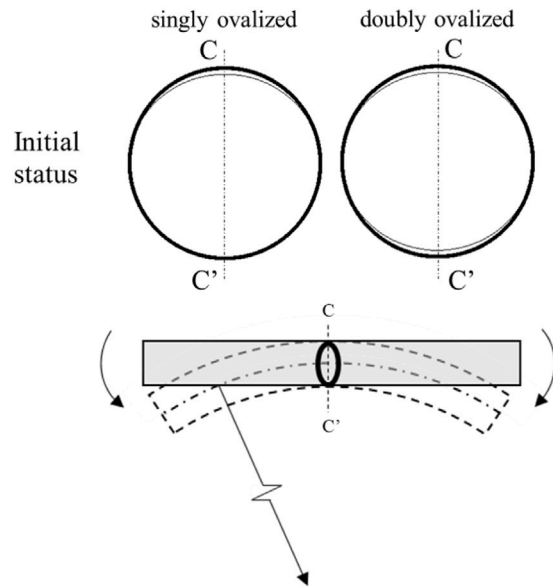
Fig. 6. Singly and doubly initial ovalization.
