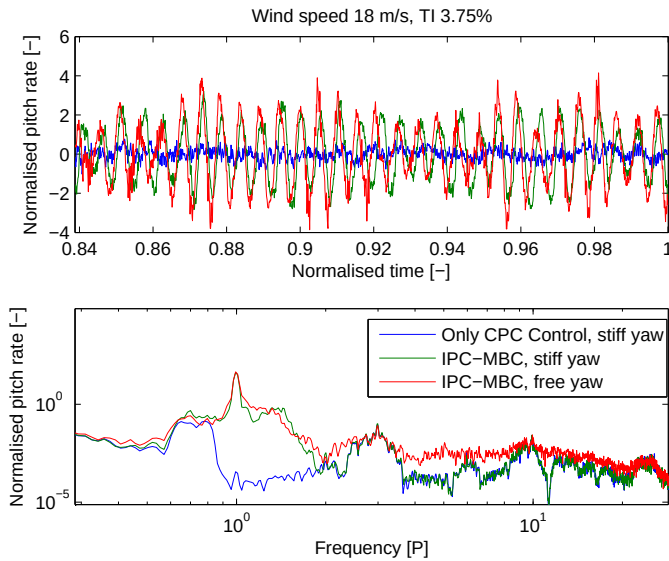
Figure 7.28: Blade pitch rate for wind speed 18 m/s, turbulence intensity 3.75%.
