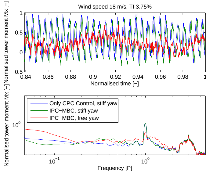
Figure 7.26: Tower side-side loads for wind speed 18 m/s, turbulence intensity 3.75%.
