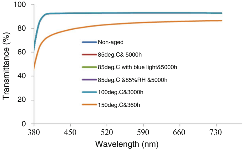
Fig. 9.6 Transmission spectra after being subjected to different aging conditions (Note: the 85 °C and 100 °C lines coincide with the nonaged line)
