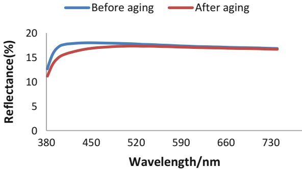
Fig. 9.17 Reflectance measured for PMMA diffuser before and after aging
