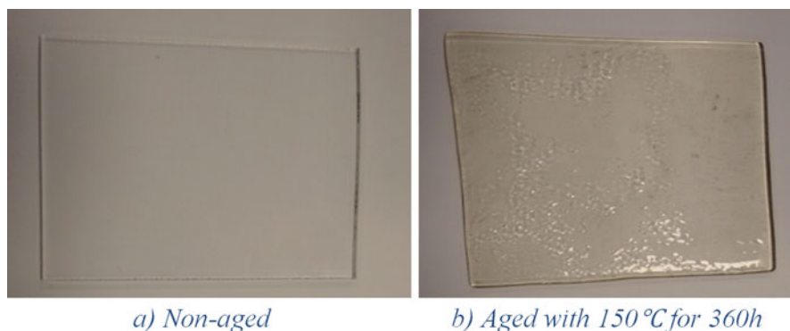
Fig. 9.5 Discoloration of PMMA after aging. (a) Nonaged. (b) Aged with 150 °C for 360 h
