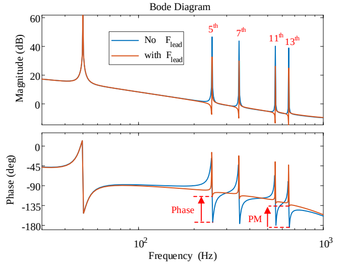
Fig. 10. Bode plot of the open-loop with harmonics resonators.
