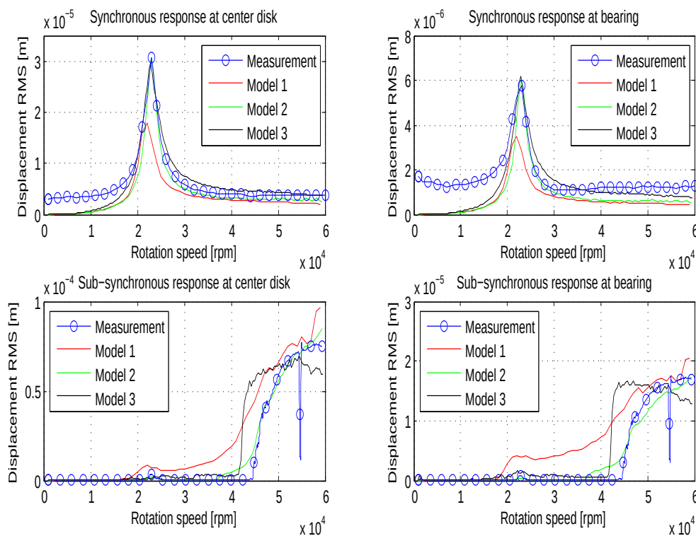
Figure 8. Synchronous and sub-synchronous rotodynamic response.
