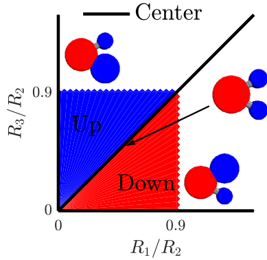
Figure 15. State diagram of the long-time y -position of trimer particles, consisting of three disks with radii R_i ( R_2 corresponding to the middle disk). The black lines indicate symmetric particles with R_1 = R_2 (symmetric trimers) and R_1 = 0 or R_3 = 0 (dimers), which move to the center of the channel. The red triangle indicates shapes that have a long-time y -position close to the lower boundary at y = -W/2 , the blue triangle indicates shapes with a long-time y -position close to the upper boundary at y = W/2 .
