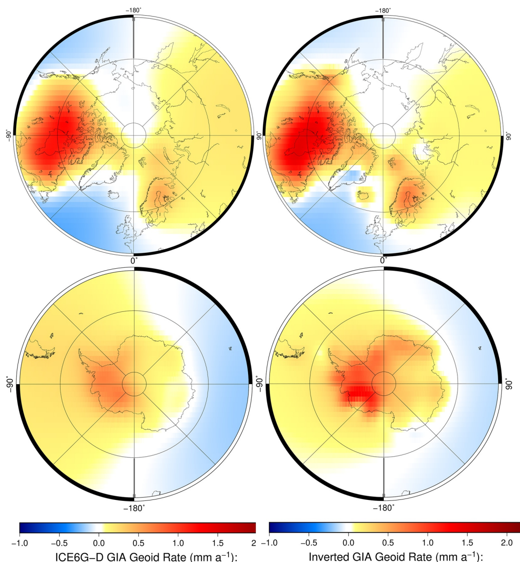
Figure 7. Comparison of GIA geoid rate in the polar regions. The left panel are plots of the ICE6G-D (Peltier et al., 2018) geoid rate in the North and South Pole. The right are two plots of our GIA inversion results in the same region. GIA, glacial isostatic adjustment.
