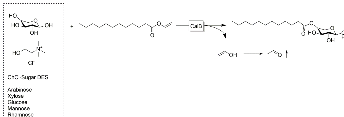
Scheme 1. Using carbohydrate-based DES as solvent for the synthesis of glycolipids.
