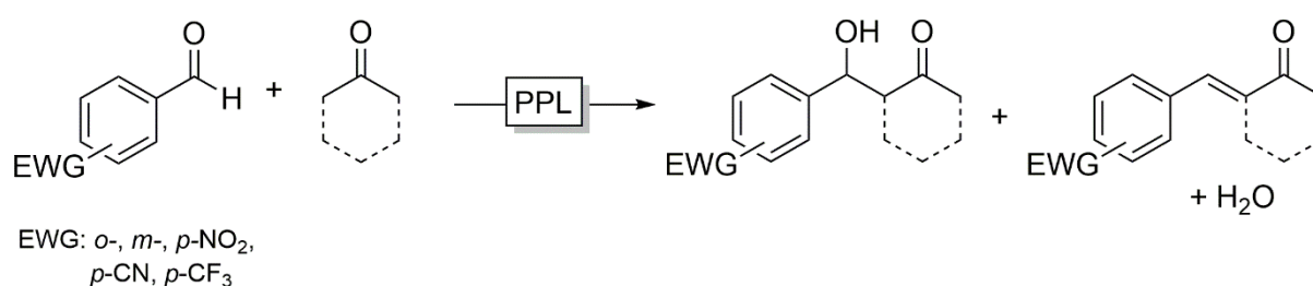
Scheme 3. Aldol reaction (condensation) catalysed by porcine pancreatic lipase (PPL) in ChCl-Gly-DES.
