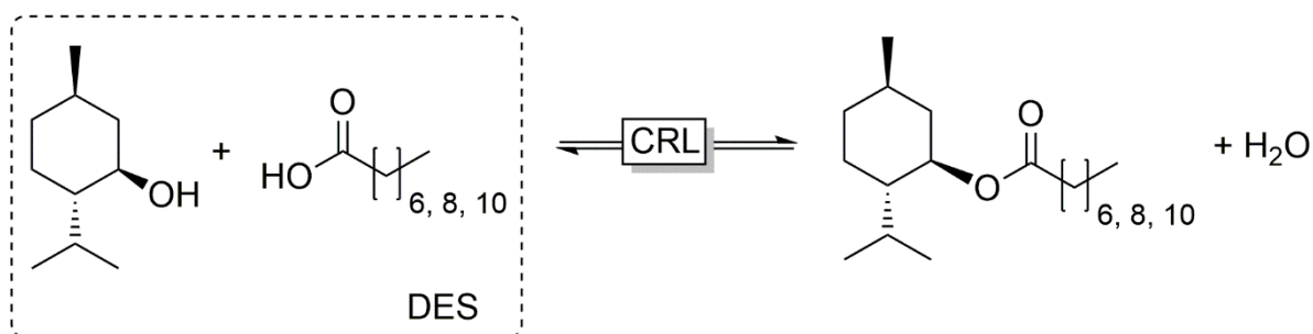
Scheme 4. Using a DES formed by menthol and fatty acids for the lipase (from Candida rugosa , CRL)-catalysed synthesis of menthol esters in a solvent-free approach.
