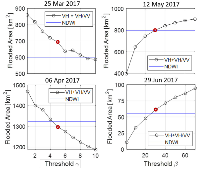
Fig. 7. Algorithm calibration. The total F area (TW + FV) is evaluated for different thresholds \gamma (left panels) during the flood expansion (March 25, 2017) and flood peak (April 6, 2017), and for different threshold \beta (right panels) during the flood recession (May 12 and June 29, 2017). The area estimated from the matching LS8 acquisitions by NDWI thresholding is also reported, and the selected thresholds ( \gamma = 5 and \beta = 30 ) are highlighted.
