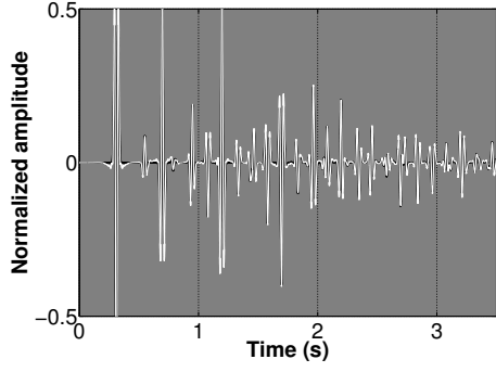
Figure 1: Virtual Green's function with free-surface multiples (white line) with virtual source \mathbf{x}_j'' at depth 1.75 km and recording at the virtual receiver \mathbf{x}_i' at depth 0.75 km for the model in Figure 2 with a free surface. The modeled Green's function is superimposed on it which also includes the free-surface multiples (black line).
