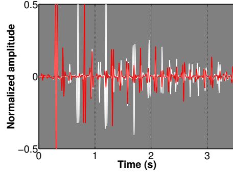
Figure 3: Virtual Green's function with virtual source \mathbf{x}_j'' at depth 1.75 m and recording at the virtual receiver \mathbf{x}_i' at depth 0.75 km retrieved by the method of this paper (white line) and computed by interferometry (red line). The retrieved virtual Green's function (white line) is almost identical to the modeled virtual Green's function.
