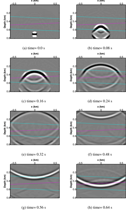
Figure 5: Snapshots of the virtual Green's function G(\mathbf{x}'_i, \mathbf{x}''_j, t) with virtual sources \mathbf{x}''_j = (0, 0.7) km and virtual receivers \mathbf{x}'_i populating the target box in Figure 4a. The dotted lines represent the velocity interface (blue) and the density interface (magenta).
