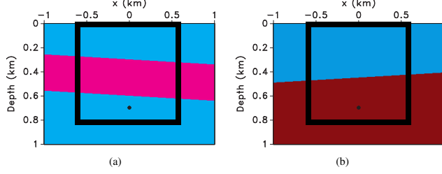
Figure 4: Synthetic model (a) velocity model with velocities ranging from 2.0 to 2.4 km/s (b) one-interface density model with densities ranging from 2.0 to 3.0 g/cm 3 . The dot shows the position of the virtual source for the virtual Green's function and the black box is the target zone where we place virtual receivers.
