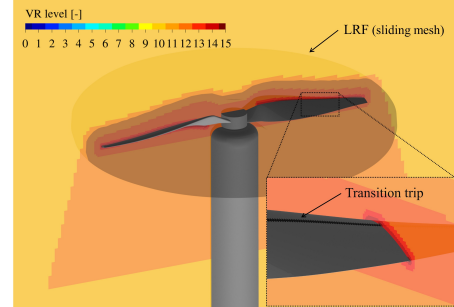
Figure 3. PowerFLOW computational setup and mesh layout.
