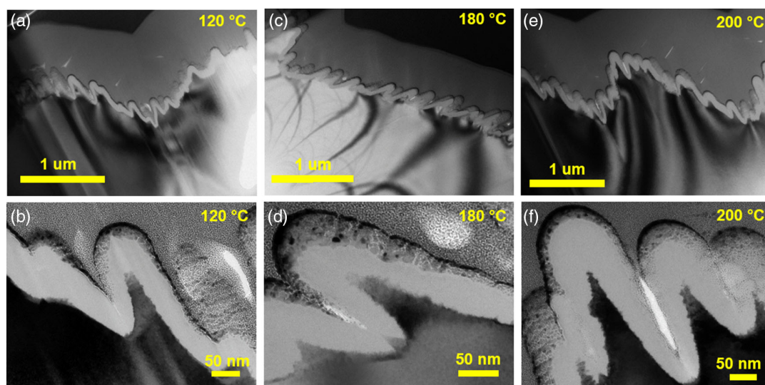
Figure 6. TEM images of a-Si:H films deposited on MST samples (Under deposition conditions of 13 \text{ mW cm}^{-2} , 0.7 mbar and R=3 ): a,b) Conformal growth under 120^\circ\text{C} . c,d) Initiation of the gap in the film at 180^\circ\text{C} . e,f) Formed gap between the film at 200^\circ\text{C} .
