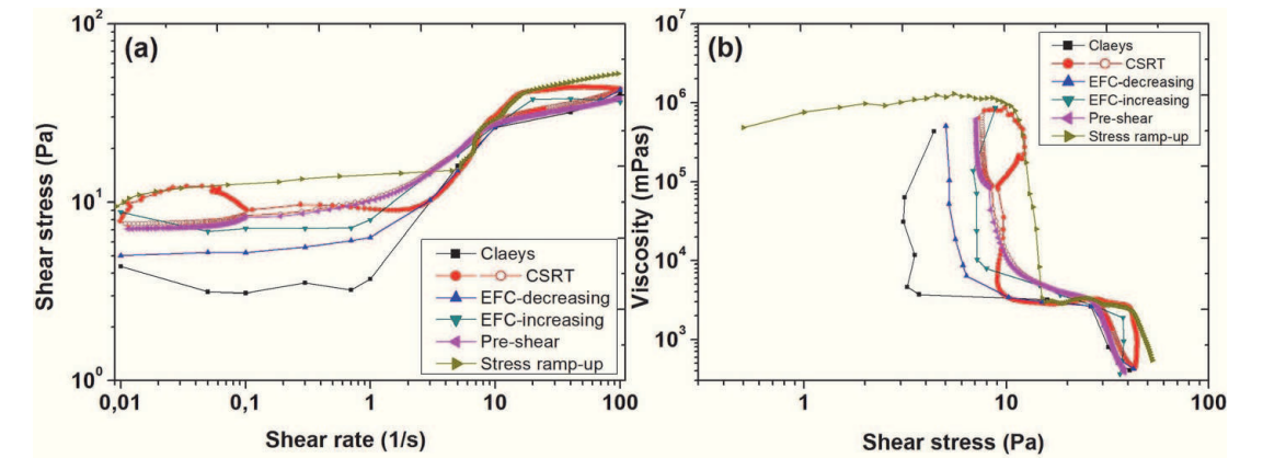
Figure 4. (a) Shear stress as a function of shear rate and (b) apparent viscosity as a function of shear stress for mud sample collected from port of Hamburg using Couette geometry; solid symbols in CSRT protocol represent the ramp-up and the empty symbols represent the ramp-down; solid lines are just the guide for the eye. Reprinted from Ref. [46].
