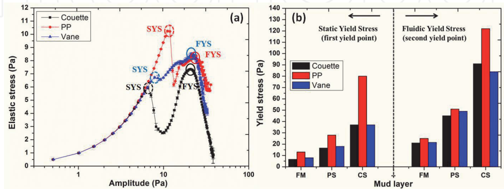
Figure 2. (a) Elastic stress as a function of amplitude at 1 Hz using different geometries for FM layer obtained from Port of Hamburg. Solid line is just a guide for the eye. Bars represent standard deviation. Circles with dashed lines represent the static yield points (SYS) and circles with solid lines represent the fluidic yield points (FYS). (b) Static and fluidic yield stress values obtained from elastic stress method for different mud layers collected from Port of Hamburg using Couette, parallel plate and vane geometries. Reprinted from Ref. [40].
