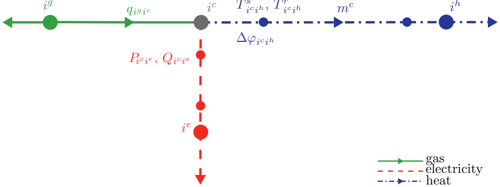
Figure 3.5: Network representation of a coupling node, showing quantities of interest for LF and the network elements they are associated with.
