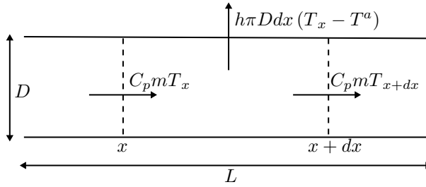
Figure 2.3: Pipe with energy flow into, and out of, a small volume of the pipe.
