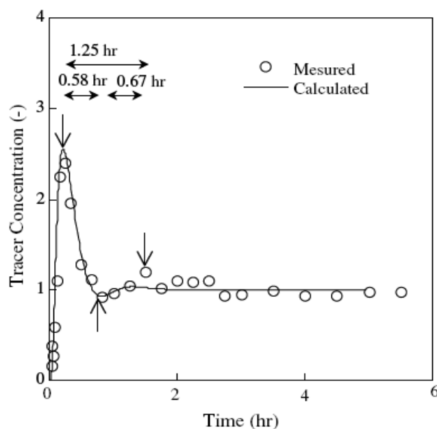
Fig. 6-2 Tracer response of experimental and simulation data (Terashima et al. 2009).
