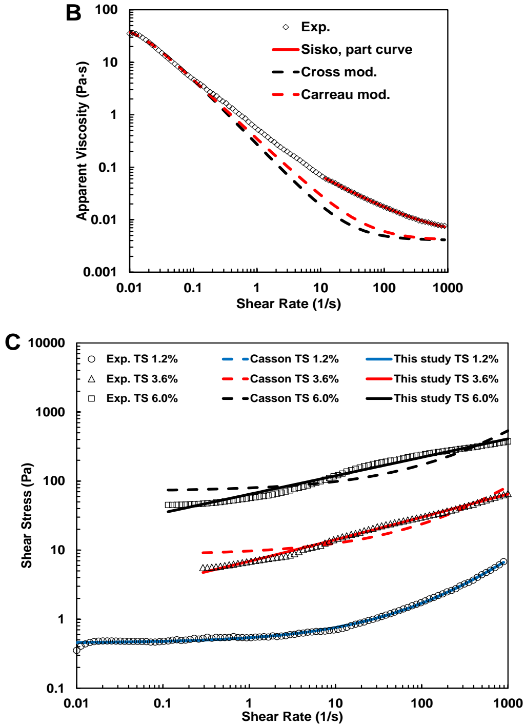
Fig. 2-2 Fitting by the models with limiting parameters, A: original and B: modified models for the GT sludge; and C: Casson and the expression in this study for the VFC sludge.
