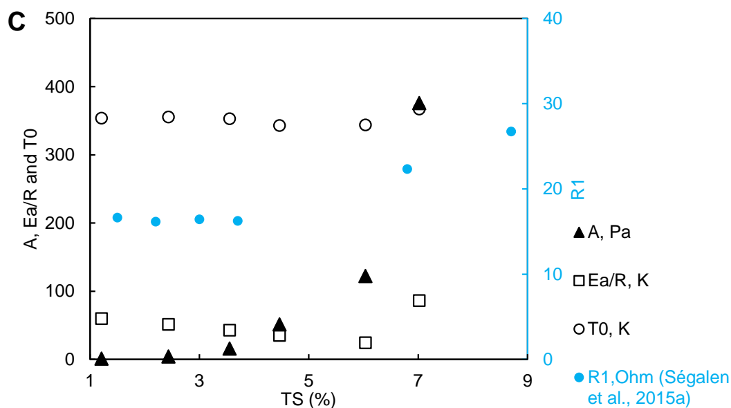
Fig. 3-3 Model correlation results. A: T_0 temperature, WAS 4.5%; B: to water dynamic viscosity, all WAS samples; and C: the VTF model parameters for \tau_0 to TS concentration, compared to experimental data (Ségalen et al., 2015a).
