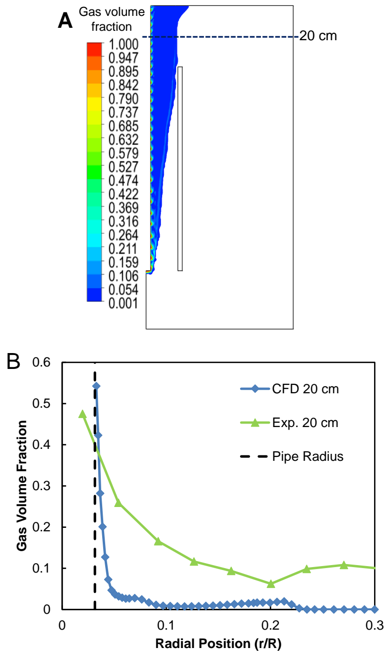
Fig. 4-7 (A) Predicted gas phase distribution in the whole domain, and (B) at 20 cm height combined with experimental data (Karim et al. 2004); gas flow rate 28.32 L/h.
