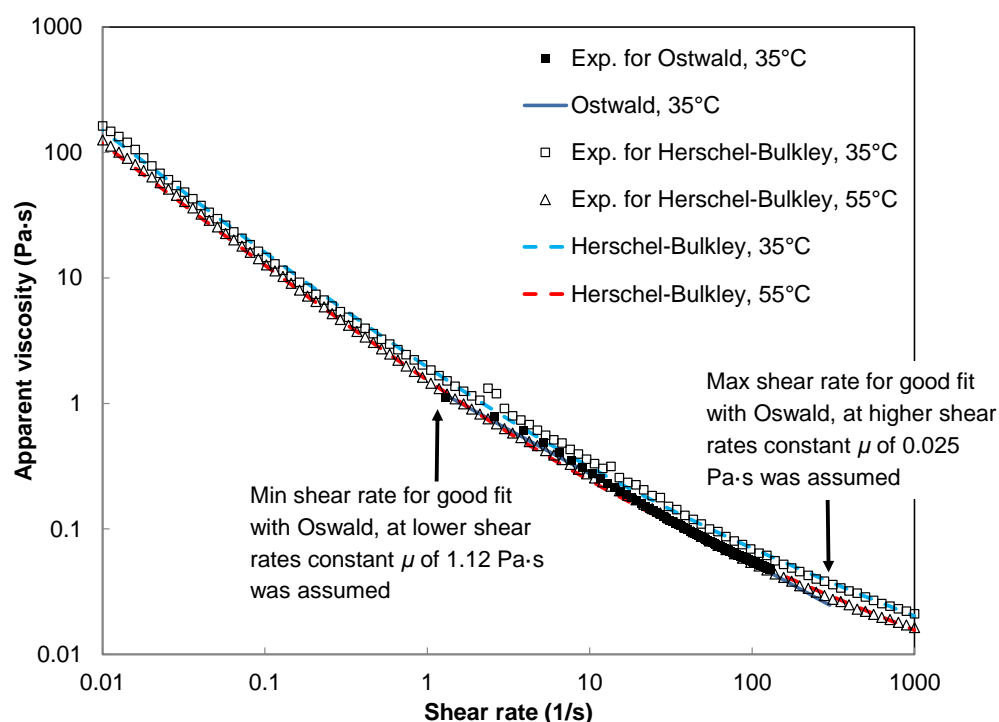
Fig. 5-2 Sludge rheological data, experimental and model fitting by Ostwald and Herschel-Bulkley.
