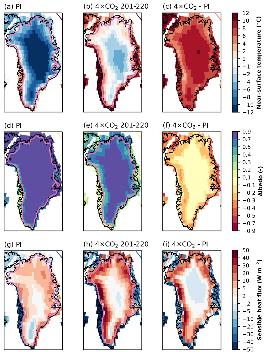
Figure 5. Simulated summer (JJA) Greenland climate from the land model CLM5 for pre-industrial forcing (first column), high atmospheric \text{CO}_2 forcing ( \text{hCO}_2 , years 201–220, second column), and difference (third column): (a–c) near-surface temperature ( ^{\circ}\text{C} ), (d–f) albedo, (g–i) sensible heat flux (positive from atmosphere to surface, \text{W m}^{-2} ). CLM5, Community Land Model Version 5.
