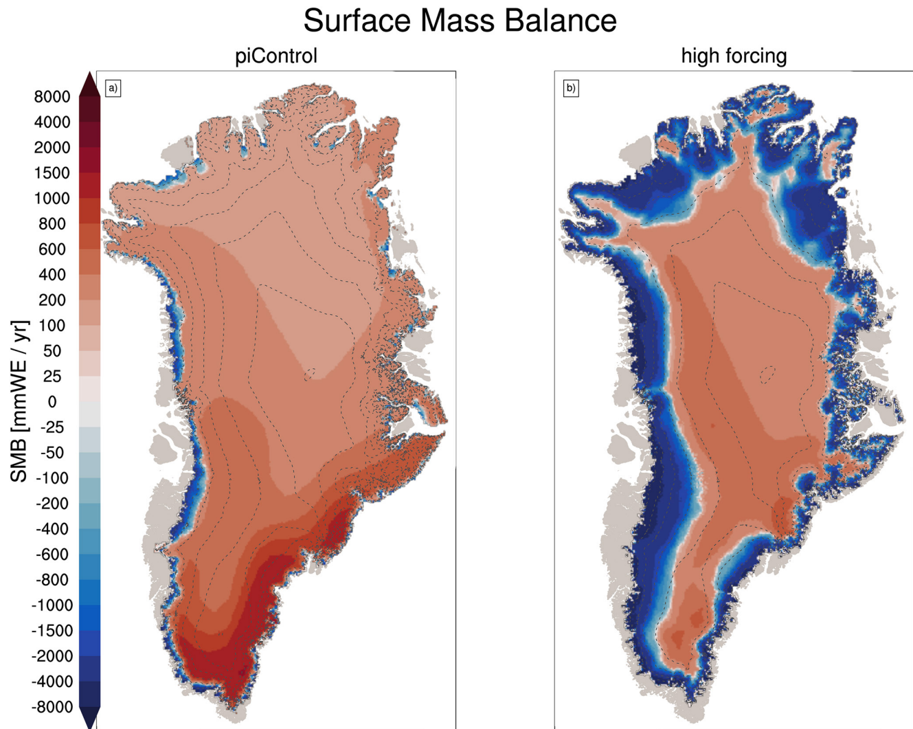
Figure 4. 20-year mean surface mass balance (mm WE yr -1 ) from the ice sheet model CISM2 for (a) pre-industrial forcing and (b) high atmospheric CO 2 forcing. Accumulation zone in red, ablation zone in blue. Dashed lines show ice sheet elevation contours at 500-m intervals. CISM2, Community Ice Sheet Model version 2.
