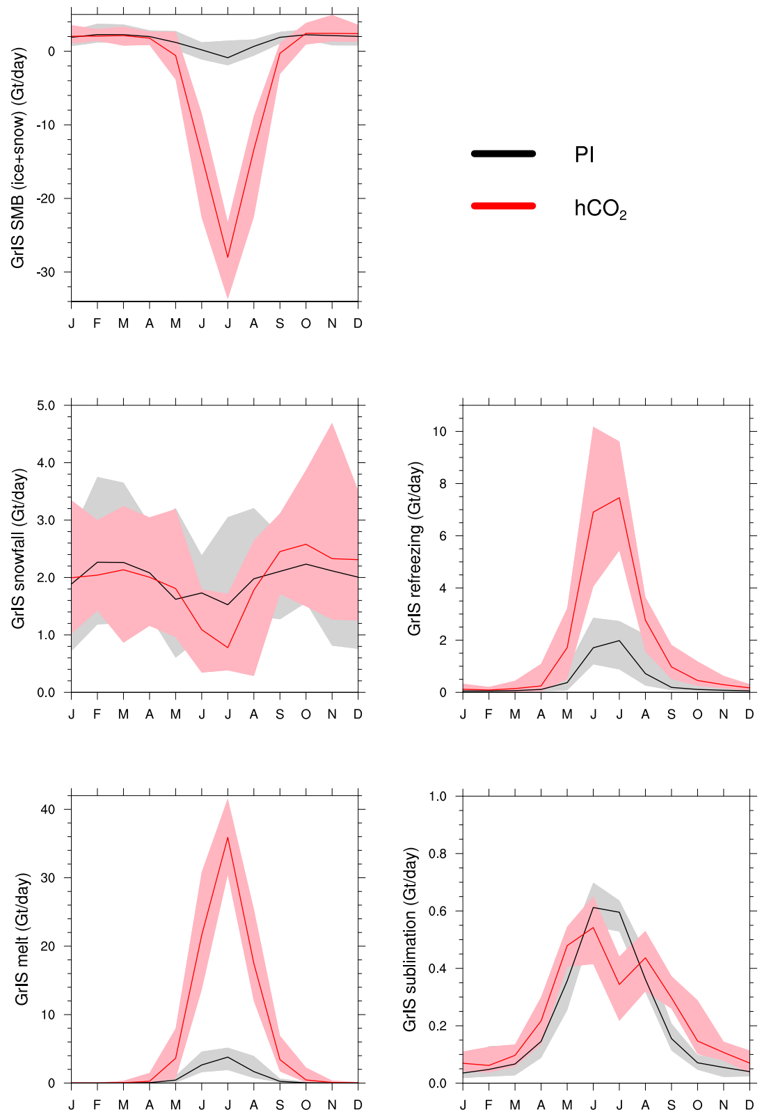
Figure 3. Climatology of the GrIS-integrated surface mass balance ( \text{Gt day}^{-1} ) and components ( \text{SMB} = \text{snowfall} + \text{refreezing} - \text{melt} - \text{sublimation} ) from the land model CLM5 for (black) pre-industrial forcing and (red) high atmospheric \text{CO}_2 forcing. Solid line is the mean, and shaded area is the range over the 20-year period. CLM5, Community Land Model Version 5; GrIS, Greenland Ice Sheet; SMB, surface mass balance.
