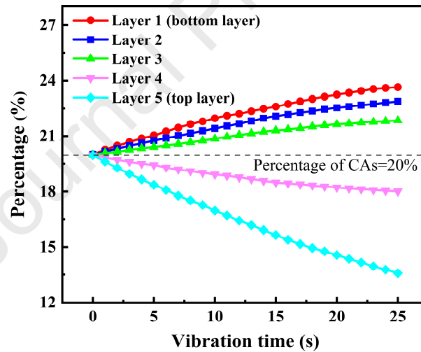
Fig. 10. The CA volume percentages of these five layers in NC.
