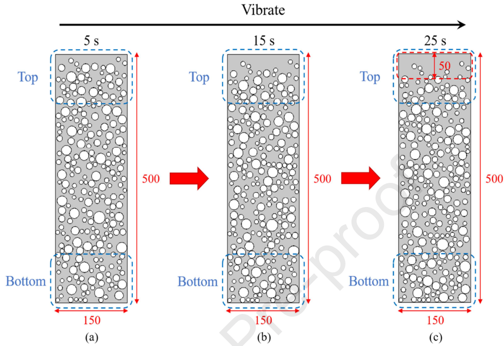
Fig. 9. Visual analysis of CA settlement under vibration (all dimensions in mm).
