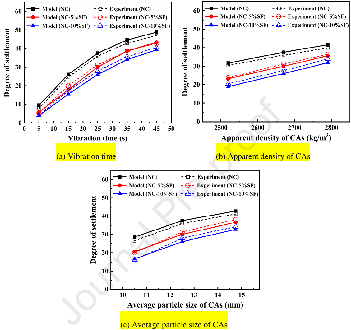
Fig. 14. Experimental verification of the prediction results.
