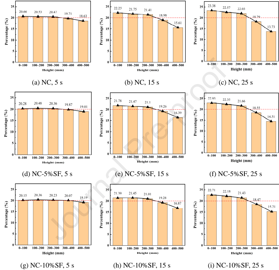
Fig. 3. Experimental results of CA settlement.
