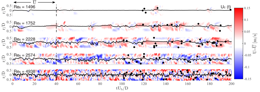
FIG. 4. Streamwise velocity patterns ( u'_x ) as a function of time for various Reynolds numbers. The concentration for this case is \phi = 0.05\% . Particles are shown only for the second part of the time series ( tU_b/D > 100 ).
