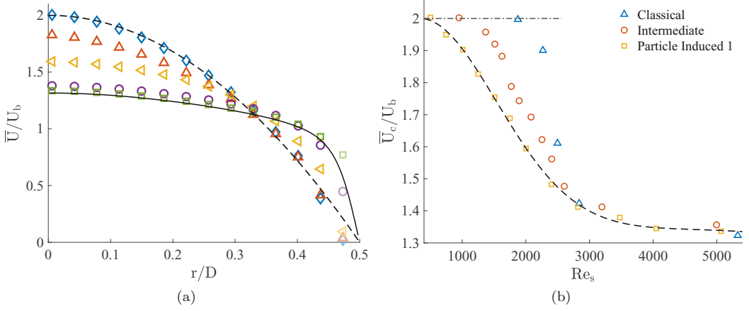
FIG. 8. (a) Average velocity profiles ( \bar{U} ), scaled with the bulk velocity for particle-induced transition ( \phi = 0.25\% ) for the following Reynolds numbers: \diamond Re_s = 500 , \triangle Re_s = 1249 , \triangleleft Re_s = 2005 , \circ Re_s = 3475 , \square Re_s = 5069 . The dashed line is the analytical solution for a laminar flow, and the continuous line is the reference data for single-phase flow with Re = 5300 . (b) Average centerline velocities scaled with the bulk velocity as a function of Re_s . The dashed line is a double Gaussian fit to indicate the trend of the particle-induced 1 transition case.
