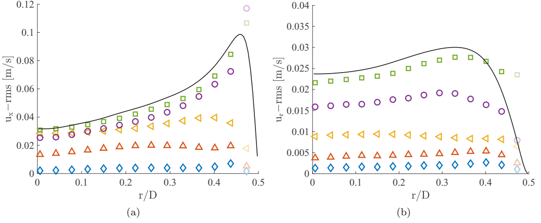
FIG. 9. (a) u_x-rms and (b) u_r-rms profiles for particle-induced transition ( \phi = 0.25\% ) and various Reynolds numbers: \diamond Re_s = 500 , \triangle Re_s = 1249 , \triangleleft Re_s = 2005 , \circ Re_s = 3475 , \square Re_s = 5069 . The continuous line represents reference data for single-phase flow for Re = 5300 .
