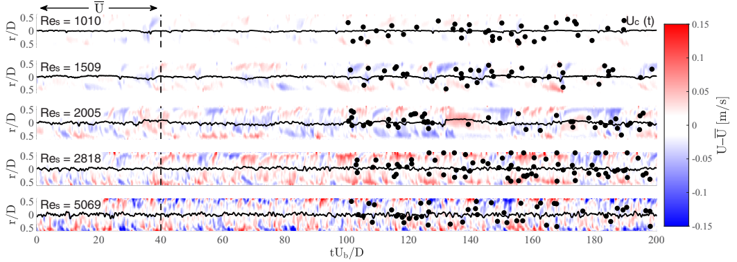
FIG. 5. Streamwise velocity patterns ( u'_x ) as a function of time for various Reynolds numbers. The concentration for this case is \phi = 0.25\% . Particles are shown only for the second part of the time series ( tU_b/D > 100 ).
