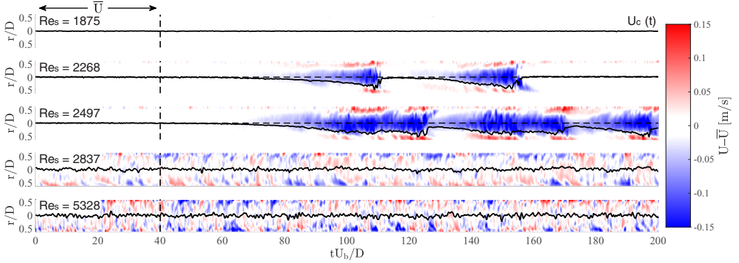
FIG. 3. Five characteristic results for a classical, single-phase transition scenario ( \phi = 0 ). The streamwise velocity patterns, u'_x , are shown as a function of dimensionless distance tU_b/D for various Reynolds numbers.
