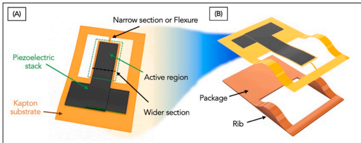
Fig. 4. (A) Design for the planar mechanism, consisting of Kapton substrate and a proper active piezoelectric area, with indication of the main parameters. (B) Exploded view of the planar mechanism on the package used in this work.
