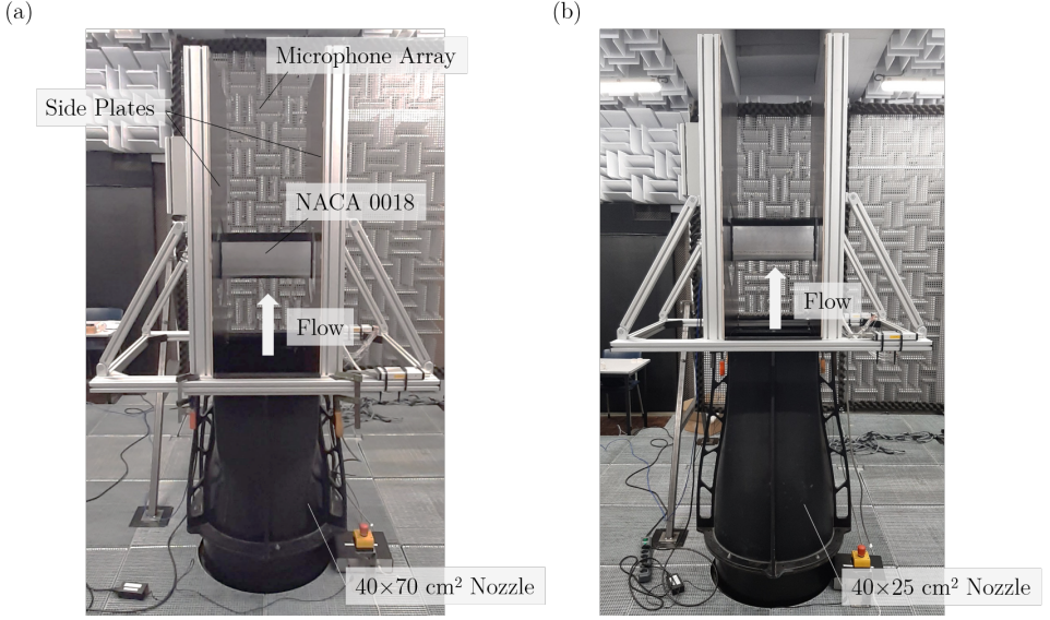
Figure 3.2: Pictures of the A-tunnel test section. The NACA 0018 model between the two side plates is shown in the foreground, while the microphone array is in the background. Air flows from bottom to top. (a) 40 \times 70 \text{cm}^2 nozzle extension. (b) 40 \times 25 \text{cm}^2 nozzle extension.
