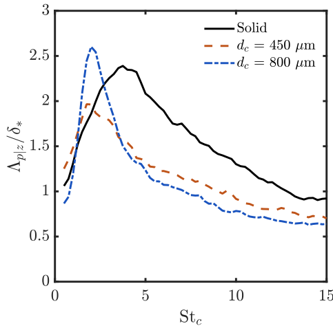
Figure 4.11: Spectral wall-pressure spanwise correlation length \Lambda_{p|z}/\delta_* as a function of dimensionless frequency St_c at a flow speed of 20 m/s.
