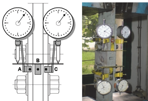
Figure 4. Test setup for friction force measurements
