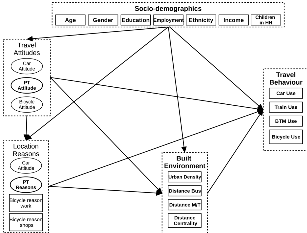
Fig. 2. Structure of the estimated cross-sectional structural equation model. Bold variables are included in the longitudinal model as well.
