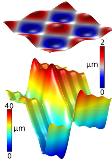
Fig. 3. The added sine-wave surface (1 μm amplitude) to the grating profile for estimation of the effect of the machining imperfections on the grating performance.
