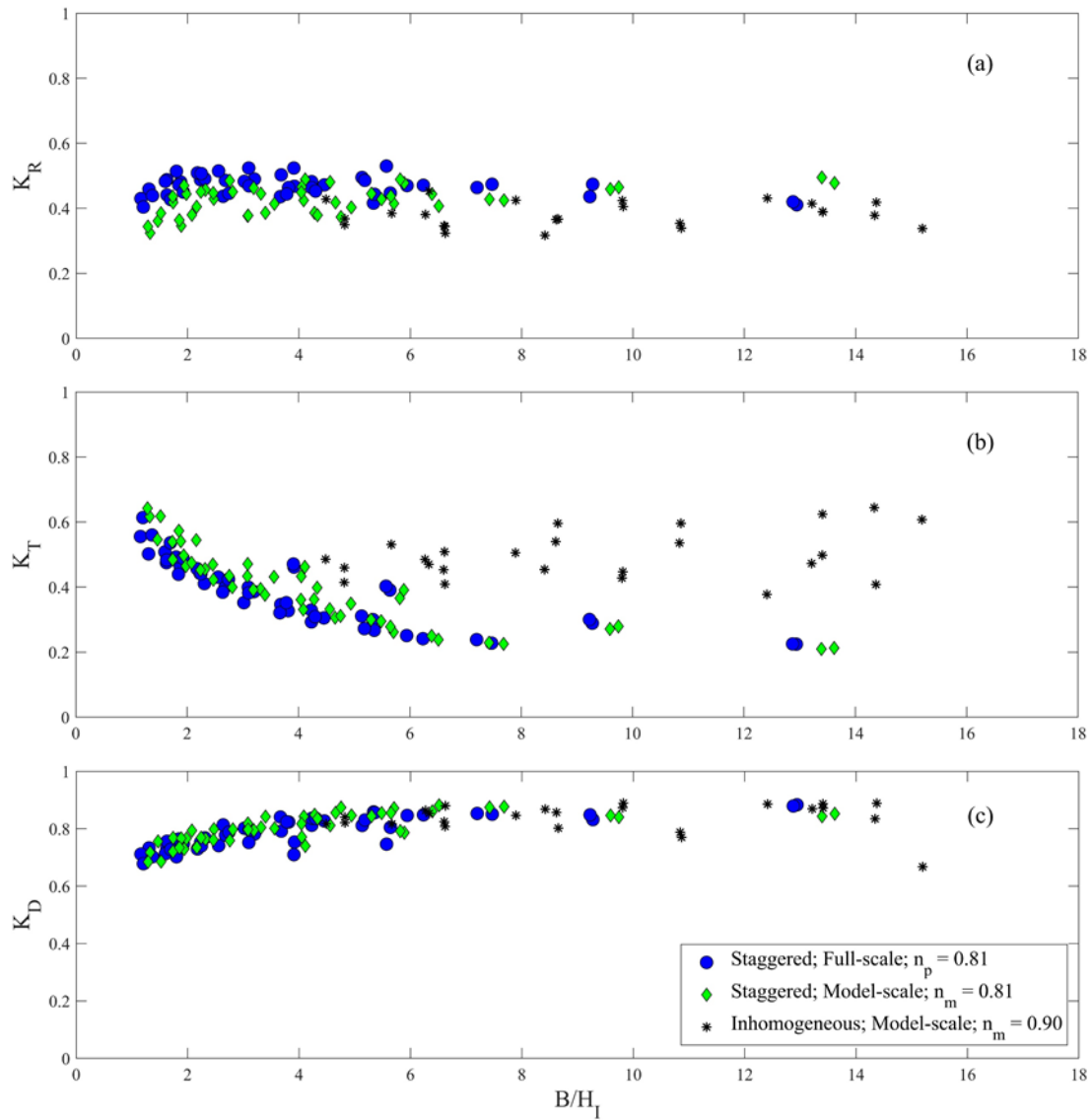
Figure 12: Relationship between reflection coefficients (a), transmission coefficient (b), and dissipation coefficient (c) and B/H_I .
