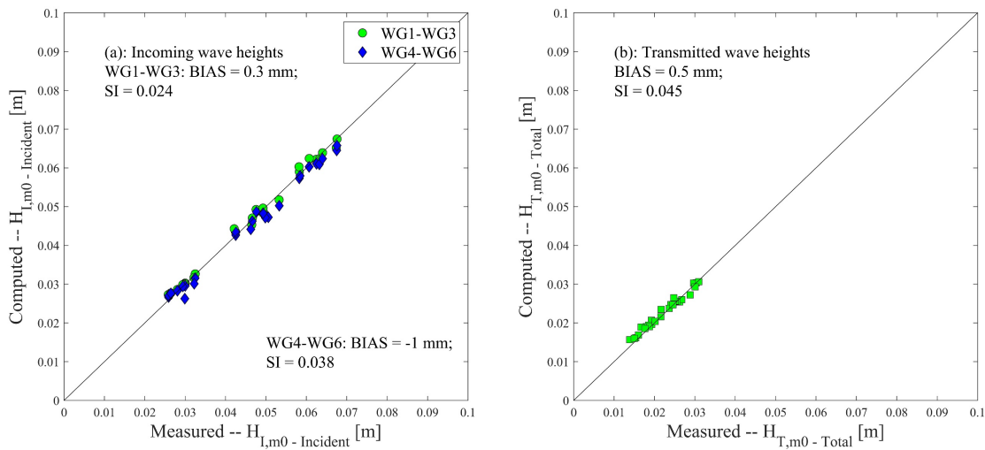
Figure 10: Comparison of wave heights between measurement and computation; (a): the incident wave heights H_{L,m0} ; (b): the transmitted wave heights ( H_{T,m0} ).
