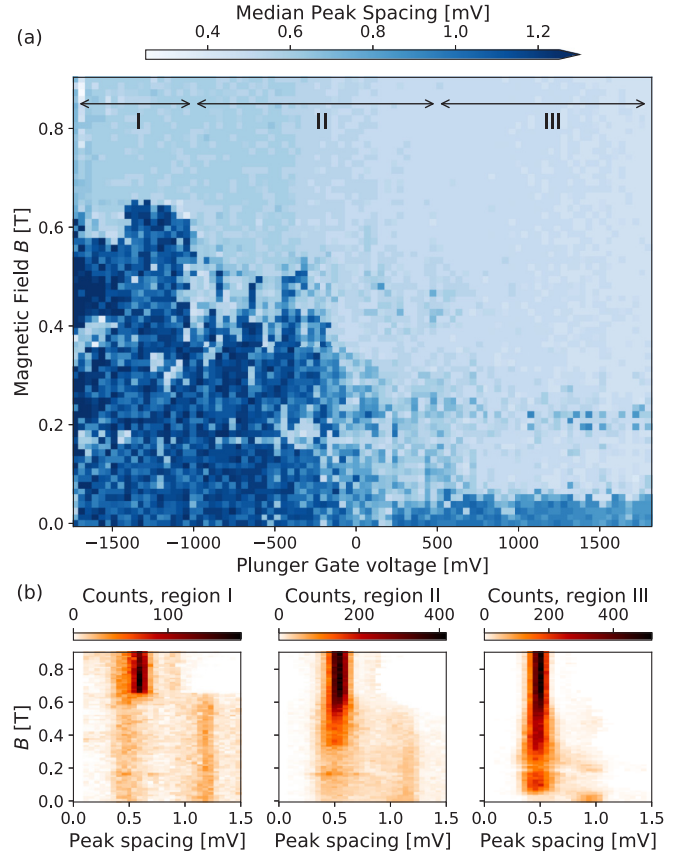
FIG. 2. (a) Median peak spacing of Coulomb blockade oscillations as a function of magnetic field and gate voltage. Dark-blue areas correspond to predominant 2e periodicity, and light blue to 1e periodicity. For each pixel, the median is determined from a window of 20 mV in plunger gate voltage, corresponding to \approx 20 –40 conductance oscillations. (b) Peak spacing distributions for regions I, II, and III as labeled in panel (a). We attribute the presence of a residual 1e peak at low B in region I to the possible poisoning of the island [11] as well as to the occasional presence of subgap states [13].
