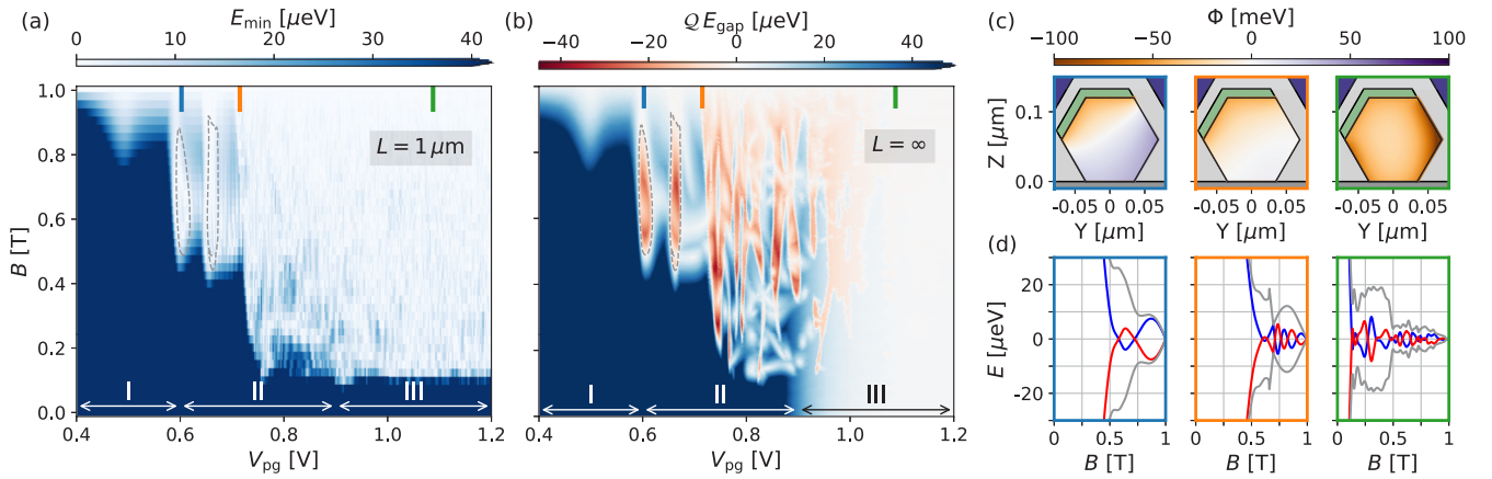
FIG. 3. (a) Quasiparticle energy gap E_{\min} as a function of plunger voltage V_{\text{pg}} and magnetic field for the simulated island of length 1 \mu\text{m} . We indicate regimes I, II, and III as in Fig. 2. The energy scale is saturated at 40 \mu\text{eV} because this is the estimated charging energy in the experimental device and thus the expected boundary at which the 2e \rightarrow 1e transition would start to occur. We note that this boundary is only weakly sensitive to the level of disorder used in the simulations, likely due to the short length of the wire [35]. (b) Bulk topological phase diagram indicating the bulk gap E_{\text{gap}} and the sign of the topological index Q = \pm 1 , both obtained via the simulation of the band structure of an infinitely long wire. Red regions are topological. Two topological regimes with large gap and small coherence length are marked by the dashed gray lines in both panels (a) and (b). (c) Electrostatic potential profiles in the nanowire cross section for the three plunger gate values indicated by blue, orange, and green bars in panels (a) and (b). (d) Magnetic field dependence of the lowest (red/blue) and first excited (gray) energy levels for three different plunger values. The left panel (blue) crosses a topological region of the phase diagram, while the two other panels (orange and green) correspond to topologically trivial regions.
