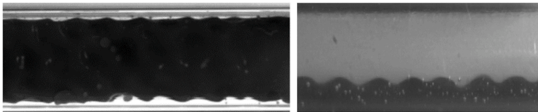
Fig. 2. Pictures from the flow experiments; (left) oil remains free from the wall (oil flow rate of 0.35 l/s and a watercut of 12%, oil density of 913 kg/m 3 and viscosity of 0.716 Pa s Van Duin, 2017); (right) oil has reached the wall (oil flow rate of 0.146 l/s and a watercut of 12.5%, oil density of 857 kg/m 3 and a viscosity of 0.411 Pa s Radhakrishnan, 2016). Note that the oil is black in the left graph and grey in the right graph.
