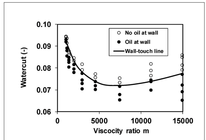
Fig. 10. The effect of the viscosity ratio on the wall-touch line for fixed pressure drop of 1100 Pa/m ( D = 21 mm).
