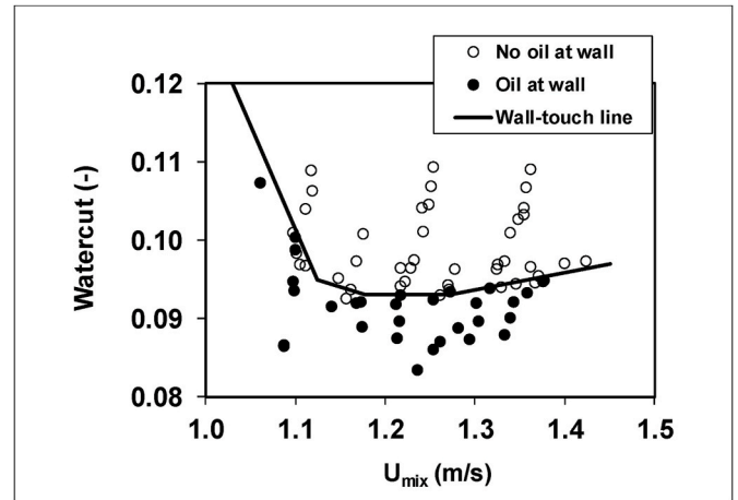
Fig. 9. The effect of the mixture velocity on the wall-touch line ( D = 21 mm, m = 1040 ).
