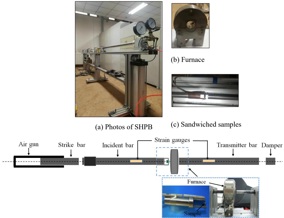
Fig. 4. Set-up for dynamic tests under elevated temperatures.
