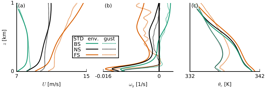
Figure 3.6: Composite profiles of (a) total wind speed U , (b) meridional vorticity \omega_y and (c) equivalent potential temperature \theta_e sampled over cold-pool gust fronts ( \theta'_e < -2 K and U' > 0 at the lowest model level; dotted lines) and the environment ( \theta'_e > -2 K), all averaged over Hours 24–36 of the STD simulations.
