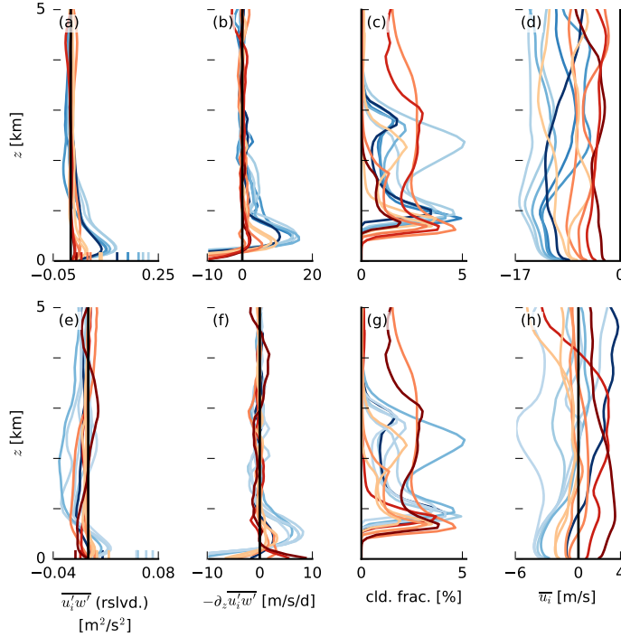
Figure 4.7: Slab-averaged daily profiles of (a, e) the momentum fluxes u'w' and v'w' , (b, f) their negative vertical divergence -\partial_z u'w' and -\partial_z v'w' , (c, g) the cloud fraction and (d, h) the zonal and meridional wind velocities. In the top row the lines are coloured by surface zonal wind velocity and in the bottom row by the surface meridional wind velocity, where blue shades indicate winter days and red shades summer days. The coloured tick marks in (a) and (e) indicate the surface momentum fluxes.
