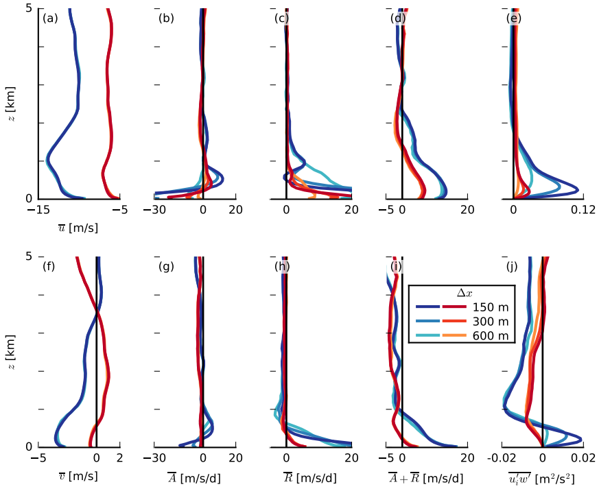
Figure 4.8: Seasonally averaged profiles of (a, f) the wind components u and v , (b, g) advection \bar{A} , (c, h) residual \bar{R} , (d, i) the sum of resolved advection and residual \bar{A} + \bar{R} and (e, j) turbulent momentum flux \overline{u'w'} for different horizontal LES resolutions \Delta x and for (a–e) the zonal wind component and (f–j) the meridional component. Blue/cyan lines depict winter and red/orange lines summer.
