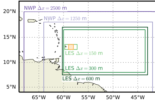
Figure 4.1: Overview of the simulation protocol of Stevens et al. (2019) with two outer domains that use NWP physics (purple) and three inner domains that use LES physics (green). The domains are coupled via a one-way nesting, and the horizontal resolution \Delta x increases as the domain size decreases. The hatched orange square indicates the area of interest of the present paper.
