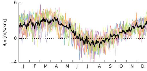
Figure 2.2: Time series of the amount of zonal shear between 1 and 3 km for the years 2008 to 2017 averaged over the area from 9^\circ to 19^\circ N and from 50^\circ to 59^\circ W (coloured lines). The black line is the average over all 10 years. The dotted horizontal line indicates 0 \text{ m/(s km)} . Data are from the ERA5 reanalysis.
