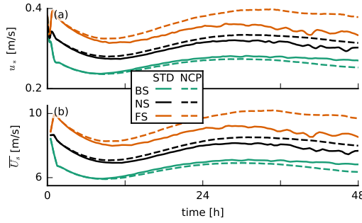
Figure 3.2: Time series of (a) the surface friction velocity u_* and (b) the domain-averaged total wind speed at 5 m height U_s . As explained in Fig. 3.1, orange indicates forward shear (FS), black no shear (NS) and green backward shear (BS), while solid lines indicate the standard (STD) runs and dashed lines the no-cold-pool (NCP) runs. The line colours and types are the same in all following figures, unless indicated otherwise.
