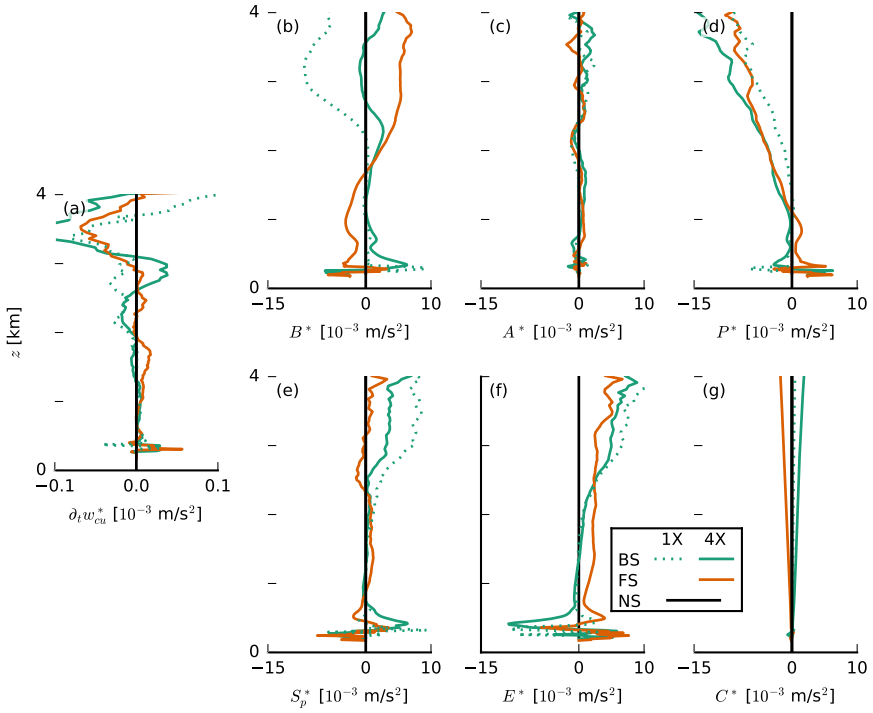
Figure 2.A1: Slab-averaged profiles (averaged from 30 to 36 h of the simulations with prescribed surfaces fluxes) of the terms of the cloudy-updraft vertical-velocity budget (Eq. 2.A1) plotted as differences from the NS case (indicated by the asterisks).
