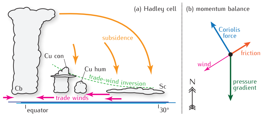
Figure 1.3: (a) Schematic of the Hadley circulation with its characterising cloud types: cumulonimbus (Cb), stratocumulus (Sc), cumulus humilis (Cu hum) and cumulus congestus (Cu con). (b) Idealised force balance of the (surface) trade-winds (in the northern hemisphere).
