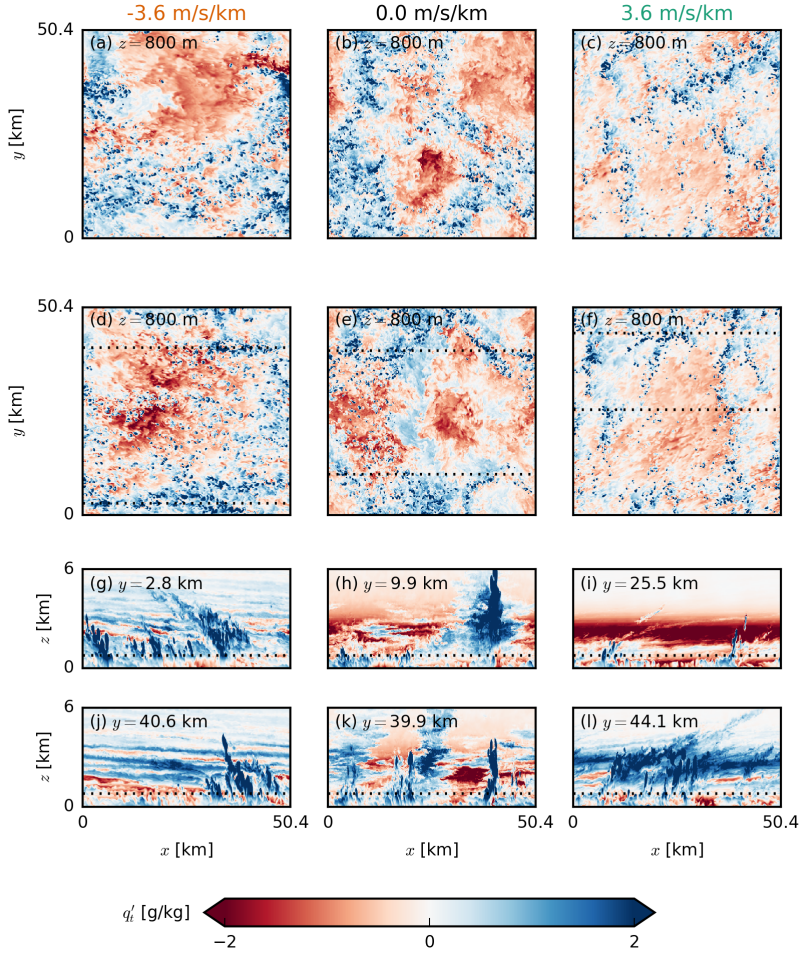
Figure 2.12: Snapshots of the LES domains of FS-4X (left), NS (centre) and BS-4X (right) exhibiting typical characteristics in the late stages of the simulations with prescribed surface fluxes. The top two rows (a–f) show horizontal x - y cross sections at two times ( t = 39.0 h and t = 46.5 h) near cloud base ( z = 800 m) of the deviations from the mean of the total water specific humidity q'_t . The bottom two rows (g–l) show corresponding vertical x - z cross sections from the lowest 6 km of the domain of the latter of the two times (d–f). The horizontal dotted lines indicate the position of the respective other cross sections.
