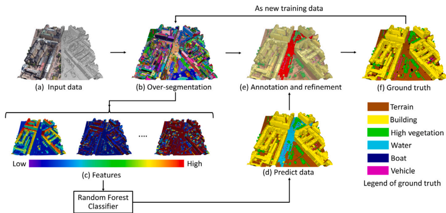
Fig. 5. The pipeline of the labelling workflow.
