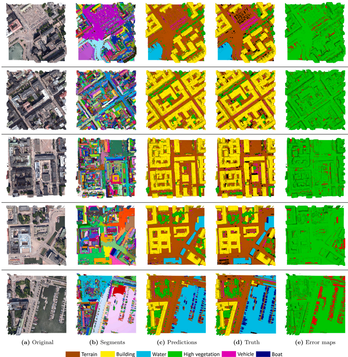
Fig. 12. Part of our semantic segmentation results. The first column shows the input texture meshes; the second column shows the over-segmentation results; the third column shows the predicted semantic meshes; the fourth column shows the ground truth meshes; the last column shows the error maps (red: errors; green: correct labels). (For interpretation of the references to colour in this figure legend, the reader is referred to the web version of this article.)
