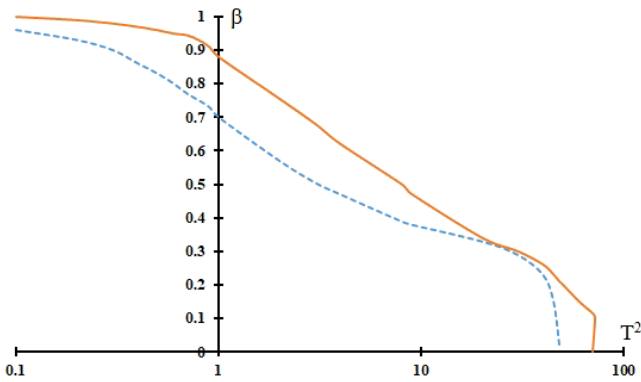
Fig. 6. Stability domains for the PLL system with time delay (42).
