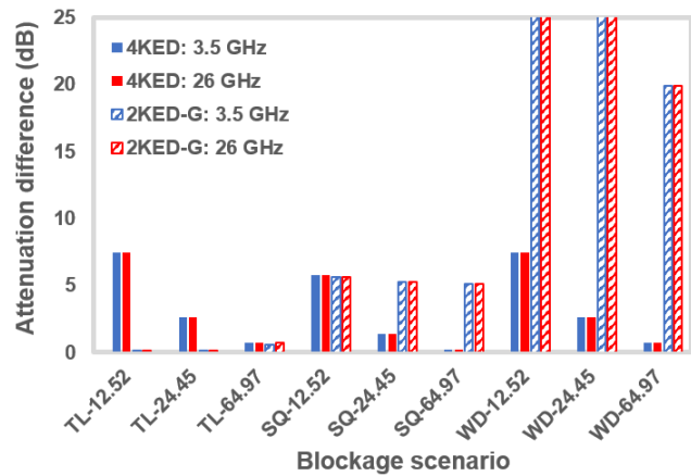
Fig. 3: Attenuation difference between 4KED-G and the other models for a blocker distanced 1 m from the TX.
