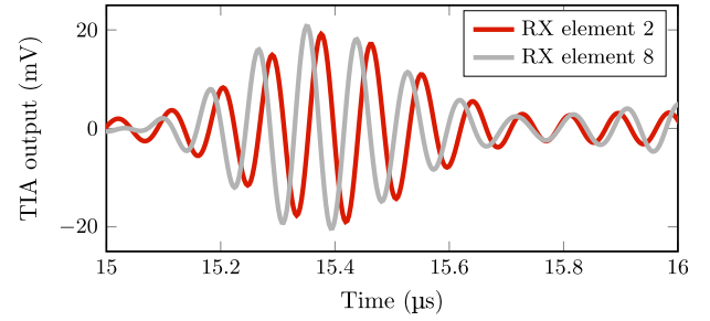
Fig. 20. Measured echo of two individual non-adjacent elements.
