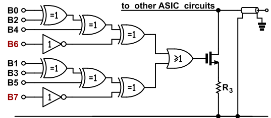
Fig. 8. Circuit used to return the CRC result to the system, where B0–B7 represent the data of one 8-bit shift register, and B6 and B7 are the CRC bits.
