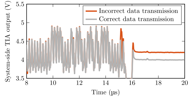
Fig. 14. TIA-output signal with a correct and an erroneous configuration data transfer.
