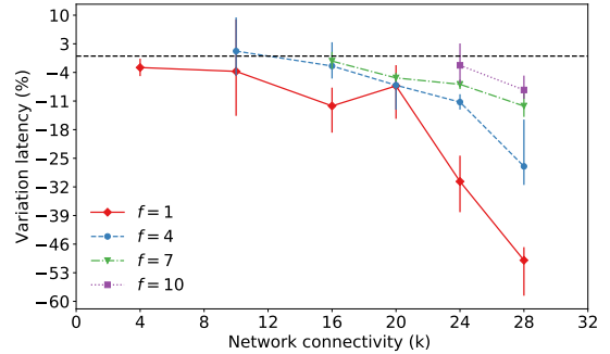
Fig. 4. MBD.4’s latency impact - N = 31 , 16KB payload.
