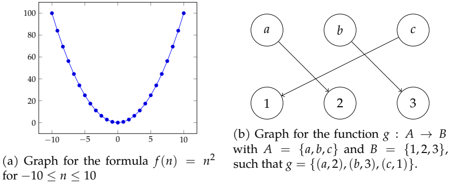
Figure 4.7: Two different graphs representing functions.
